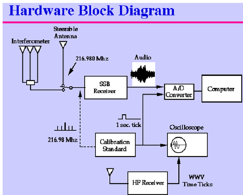
Fig. 4. Schematic of the hardware block diagram for a radar receiver [2].
