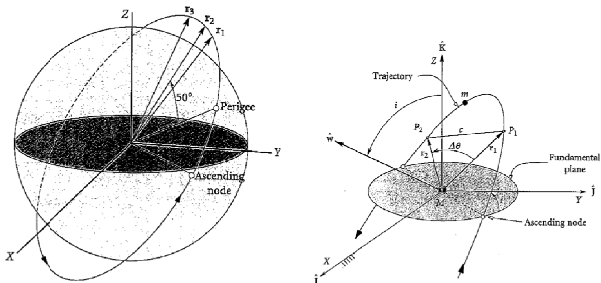
Fig. 3. Determining orbits from metric measurements. Images taken from Orbital Mechanics for Engineering Students , by Howard D. Curtis [1].
