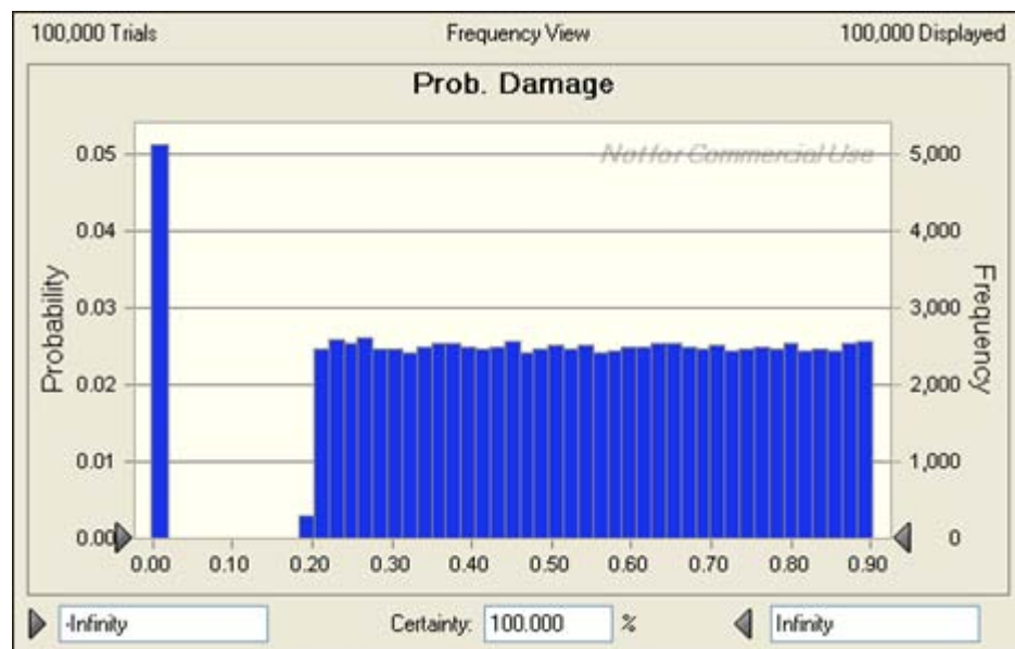
Figure 20. Frequency Plot of Monte Carlo Simulation Output
