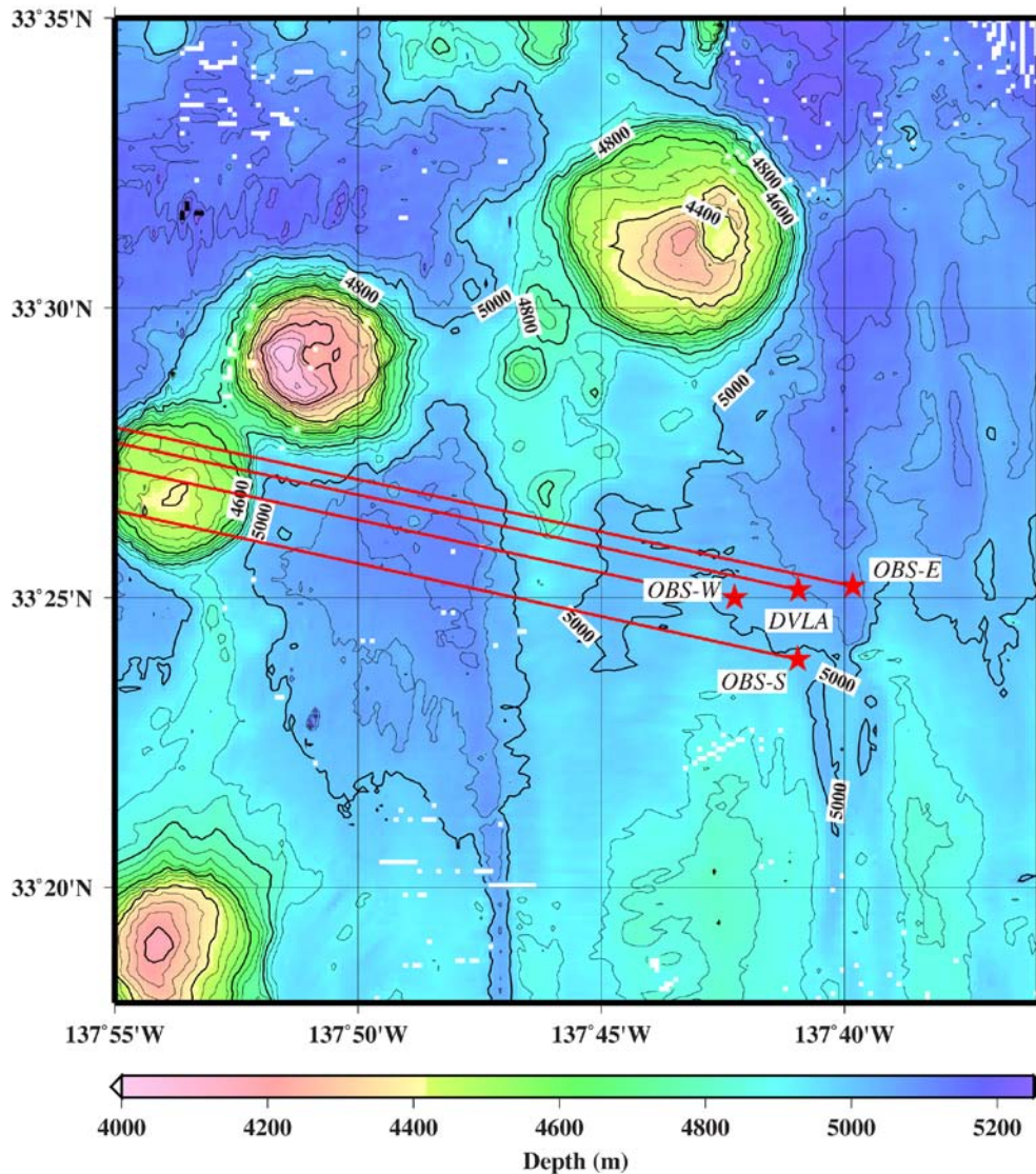
Figure 2: This figure shows the locations of the three OBSs and the DVLA with their geodetic paths to the source locations. The paths are collinear within 3km. The swath map bathymetry (Worcester, 2005) shows that all three paths pass over a seamount on the seafloor that is deeper than 4400m. Could the unexplained arrivals be scattering from this deep seamount or side-scattering from the others, which rise to about 4000m?
