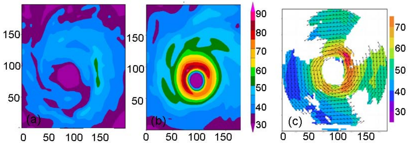
Figure 5: COAMPS-TC 3-km domain 72-h forecast surface wind speed ( m s^{-1} ) using the original COAMPS-TC version (a) and the new version (b) of the model. The Doppler radar observation is show in (c) (Courtesy of R. Rogers of Hurricane Research Division of NOAA).
