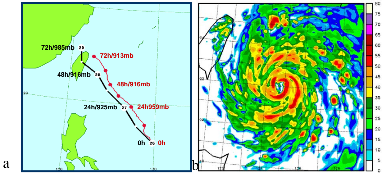
Figure 7: COAMPS-TC real time forecast initialized on 00Z 26 September 2008 for super-Typhoon Jangmi. The 72-h forecast tropical cyclone track (red) and best track (black) are shown in (a) along with the estimated central pressures and model predicted central pressure. The dots represent the tropical cyclone position at a 12-h interval. The larger white circles in the best track indicate the 00Z position with the date denoted in the circle. The model forecasted radar reflectivity at 2 km valid at 00Z 28 September (48 h) for the 5 km mesh is shown in (b).
