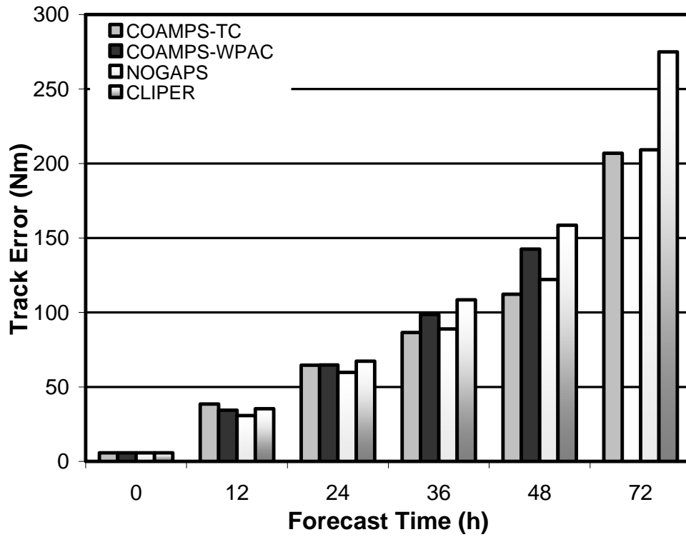
Figure 9. Tropical cyclone track error statistics for COAMPS-TC, COAMPS-WPAC, NOGAPS, and CLIPER.
