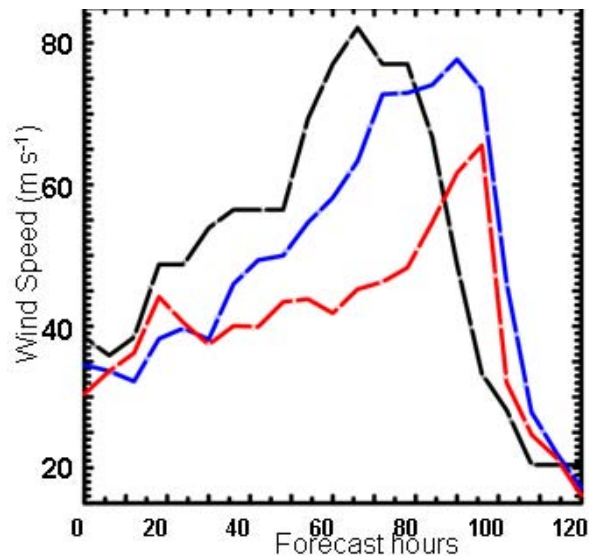
Figure 3: COAMPS forecast surface maximum winds in the 3-km resolution domain for Katrina initialized at 0000 UTC 26 August 2005 with (blue) and without (red) the sea spray parameterization. The best track is shown in black.
