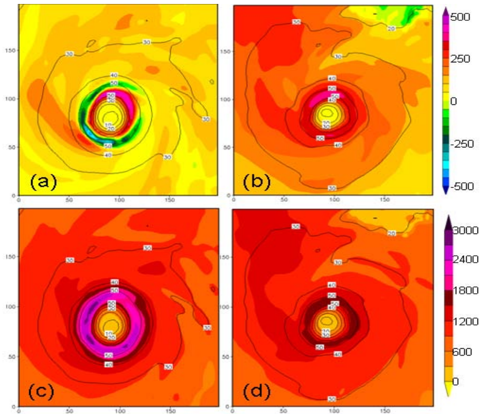
Figure 4: COAMPS 3-km resolution domain 72-h forecast surface sensible heat flux ( W m^{-2} ) with sea spray (a) and without sea spray (b), and latent heat flux ( W m^{-2} ) with sea spray (c) and without (d) valid at 0000 UTC 29 August for hurricane Katrina.
