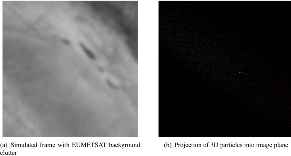
Figure 6. Projection of 3D particles (after 50 sec.) into the image plane for a simulated target against EUMETSAT background clutter ( SCR = 1/1000 ) with simulated sensor noise ( SNR = 1/6 ).
