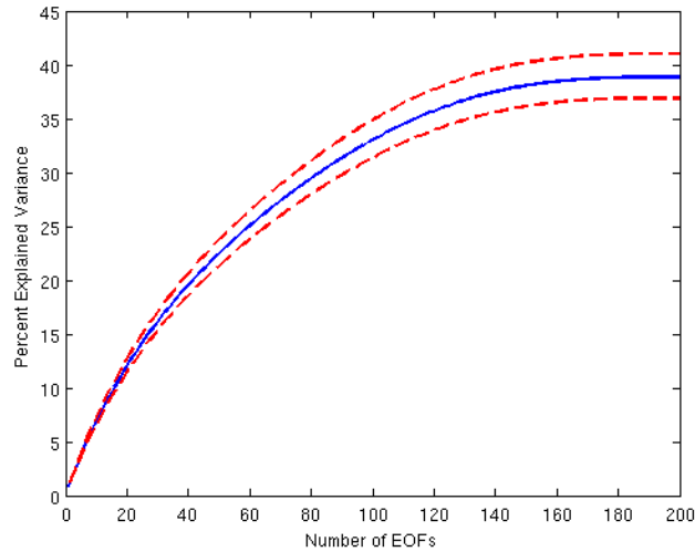
Figure 4: The cumulative percentage explained variance (blue curve) by the first 200 EOFs of the expected analysis error covariance matrix for a representative assimilation cycle in the California Current system. The red curves indicate the range of uncertainty associated with the estimate of the trace of \mathbf{E}^a .
