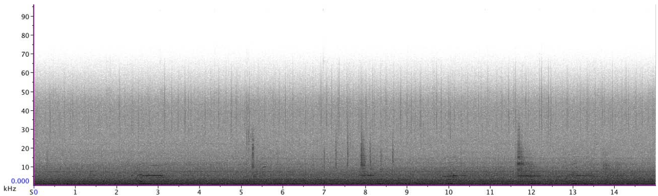
Figure 4. Spectrogram from dive 3 of SG022's deployment within about 2km of killer whales ( Orcinus orca ) off San Juan Island, WA, 4SEP2009. The analog hydrophone signal was digitized at approximately 192k samples per second. Note killer whale calls centered around 5kHz starting at t=2.5s , and click trains, low-rate, then high-rate, then low-rate, centered around 20kHz, between t=7s and t=9s .
