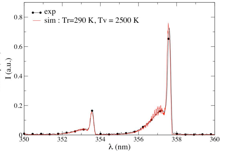
Figure 2: \text{N}_2^+ First Negative system emission spectra
