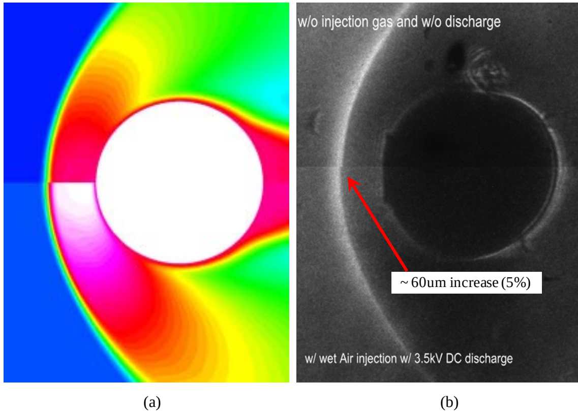
Figs. 5. Comparisons of bow shock stand-off distances without VT relaxer (top) and with VT relaxer (bottom) in vibrationally excited M=5 nitrogen flow at T=350 K and T_v=1700 K. (a): Temperature distributions predicted by CFD with VT relaxer of 3% hydrogen. (b): Density gradient distributions measured in the Shlieren method with VT relaxer of 0.1% water vapor.
