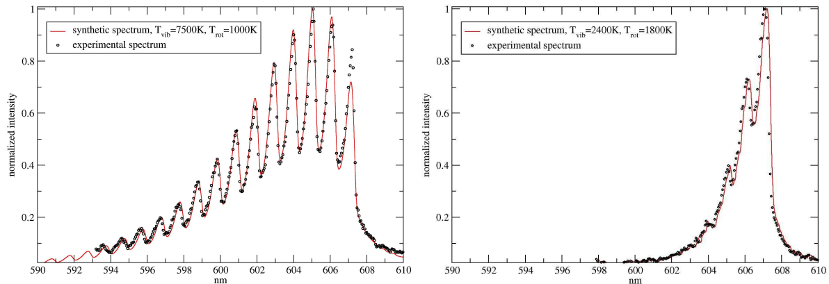
Figure 1 : comparison of synthetic and experimental (average of 2000 shots) spectra of N 2 , 150 ns (left) and 50 \mu s (right) after the discharge
