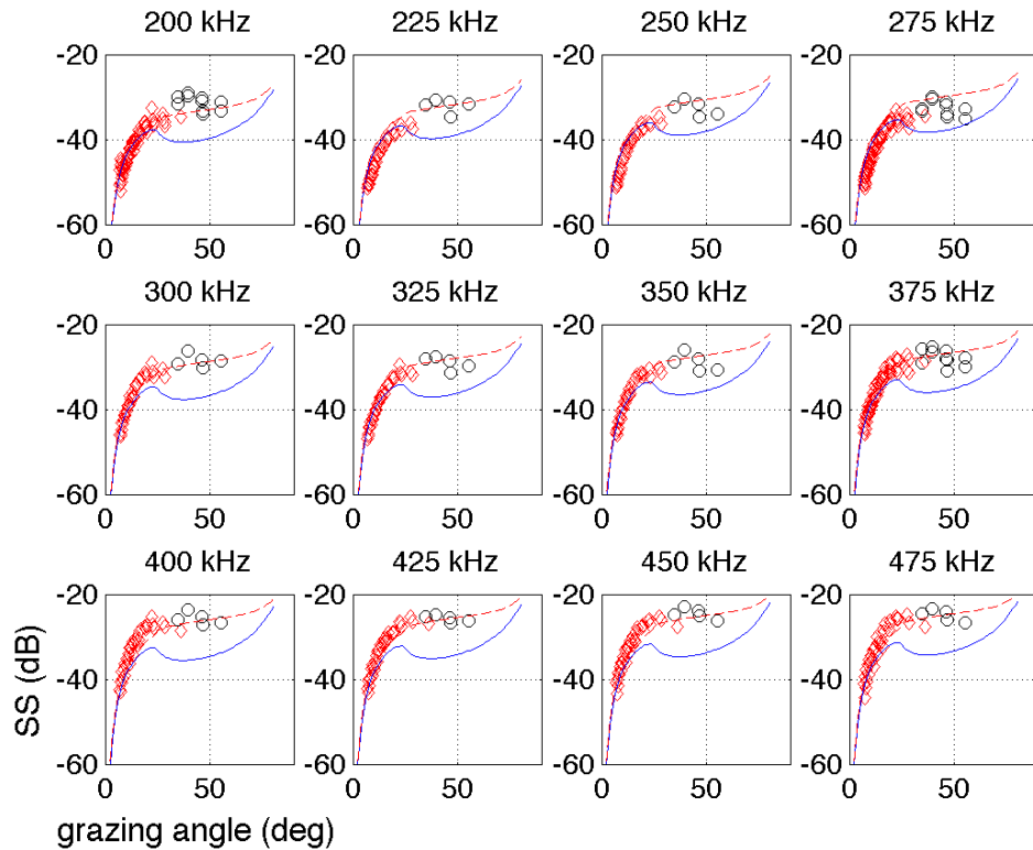
Figure 4. Data collected from the artificially smoothed sediment in the NSW pond. The red and black circles indicate different height settings for the transducers. The blue lines are predictions of perturbation theory using the roughness spectra measured using the Laser-Line Scanner. The red dashed curves are a fit to the data assuming volume heterogeneities in the density and sound speed of the sediment.
