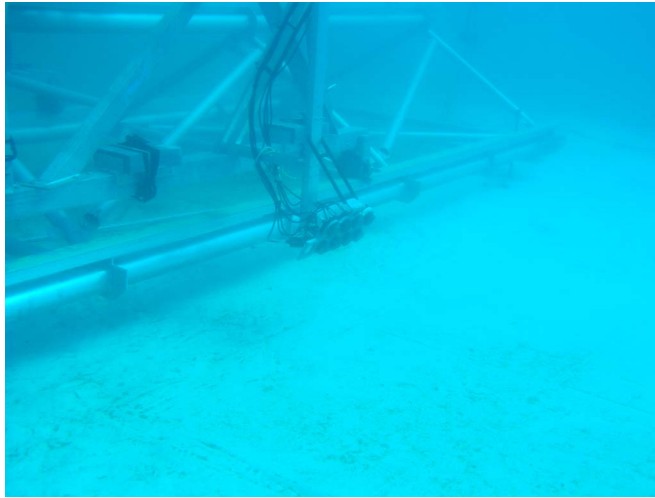
Figure 1. The scattering array mounted on the front of the APL-UW rail tower. The sediment in front of the rail was smoothed from the rail out to 5 m to minimize the scattering from the sediment roughness.
