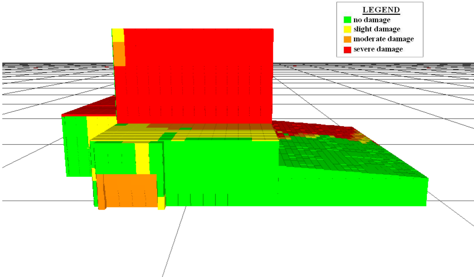
Figure 14. Damage Plot, MPPF West Face
