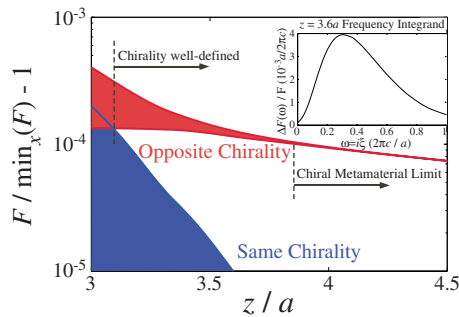
FIG. 4. (Color online) Forces (in dilute approximation) between chiral media from Fig. 3 for the SC (blue) and OC (red) cases. The range of the force across all transverse ( x ) displacements is shaded and normalized by the minimum of the force over all x . For z \lesssim 3.1a , chirality is not well defined (curves overlap). Only when curves are distinct and x independent can the systems be described as chiral metamaterials. Inset: frequency integrand of the relative force difference at z=3.6a . The smallness of the \omega=0 term is an indicator that this difference is due to chirality and not anisotropy (see text).
