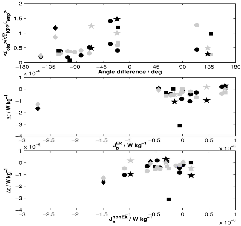
Figure 3: Comparison of \langle \varepsilon_{obs} \rangle and the KPP TKE production prediction \langle \Psi_{KPP} \rangle (black symbols) and with the empirical \langle \varepsilon_{emp} \rangle (gray symbols) of Lombardo and Gregg (1989). (top) The ratio of observed dissipation rate to predicted values vs. angle from front to wind vector direction. (middle) Differences between observed and predicted dissipations against buoyancy flux due to Ekman transport. (bottom) Differences between observed and predicted dissipations against buoyancy flux due to wind transport without earth rotation.
