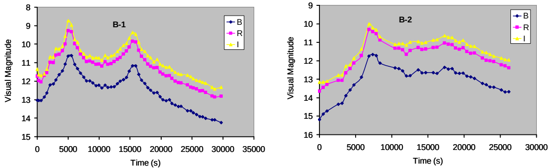
Figure 4.2a: Johnson BVRI Signatures for RSO B-1 and B-2
