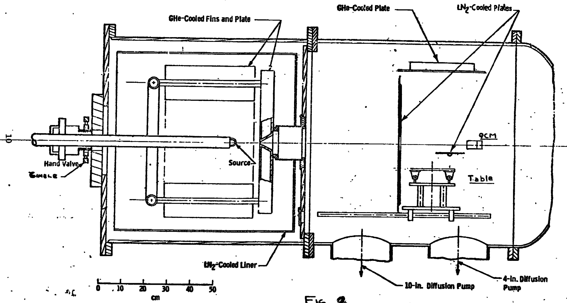
FIG. 2 MOLECULAR BEAM CHAMBER
