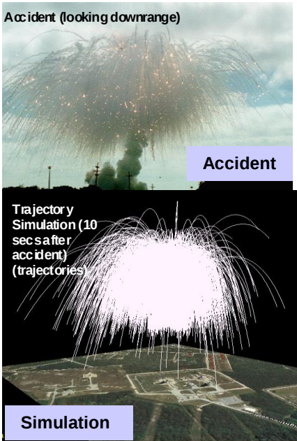
1997 T+14 explosion of a Delta II
