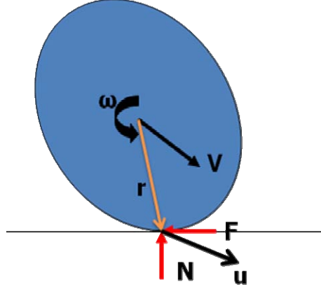
Figure 1. Fragment impact on a surface
