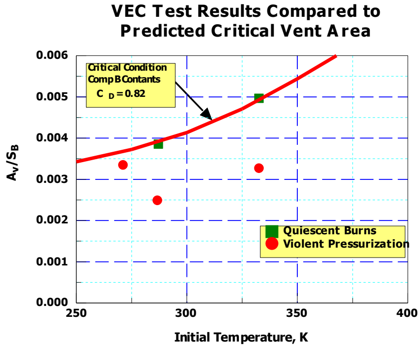
Figure 2. NWC VEC Test Results Compared to Predicted Critical Vent Area for S_B = 11.04 \text{ in}^2 .
