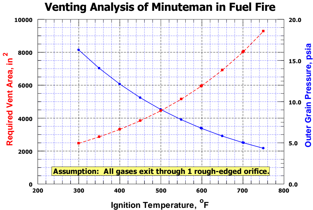
Figure 5. Effect of Ignition at Various Temperatures on Required Vent Area and Outer Grain Pressure.
