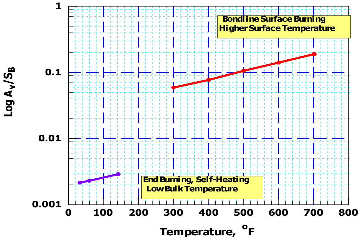
Vent Area Ratios vs. Temperature
