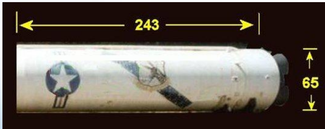
Minuteman III First Stage Motor
