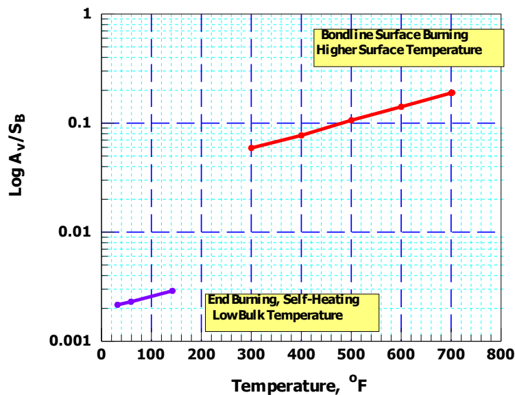
Figure 7. Comparison of required vent area to burning surface area ratios
