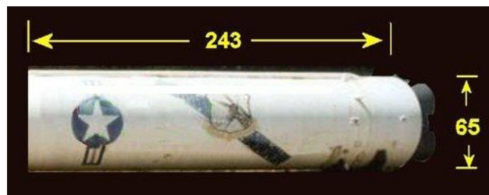
Figure 4: Minuteman III First Stage Motor
