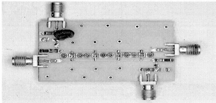
Figure 9: GaAs MESFET Distributed Amplifier Assembly
