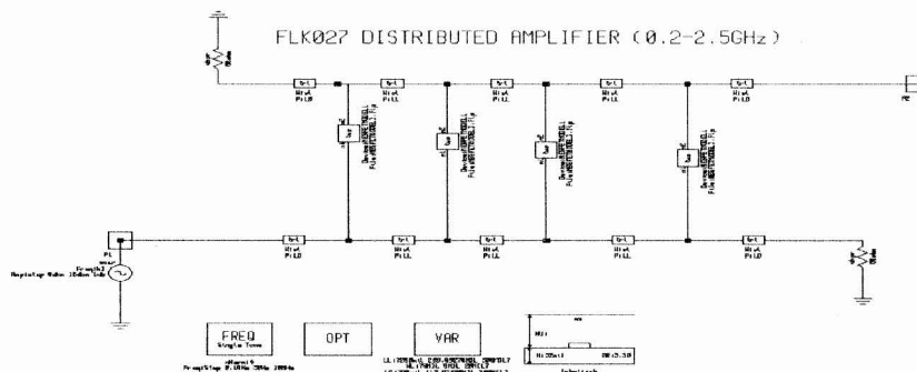
Figure 7: Schematic of GaAs MESFET Distributed Amplifier
