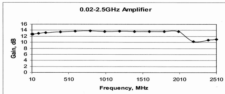
Figure 12: Gain Performance of GaAS MESFET Distributed Amplifier
