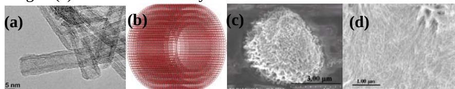
Figure 1: (a) TEM image of titania nanotubes revealing the multilayered tubular structure with inner diameters of 5-6 nm, outer diameters of 10-12 nm, and interlayer spacing of 8.7Å. (b) a structural model of multilayered titania nanotubes. (c) SEM image of a particulate of aggregated titania nanotubes. (d) Zoomed in SEM image of the particulate revealing the porous nature of the aggregated titania nanotubes.
