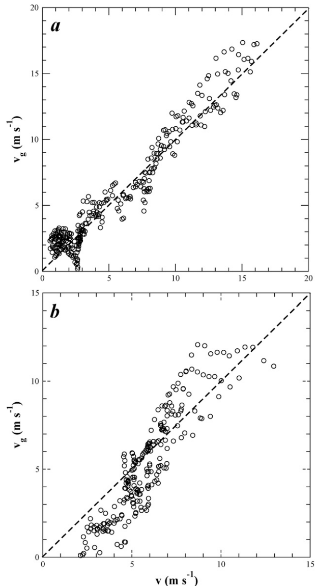
FIG. 13. Plot of the meridional geostrophic winds vs the meridional winds for set 1 parcels derived from (a) the strong-forcing case and (b) the weak-forcing case, respectively.
