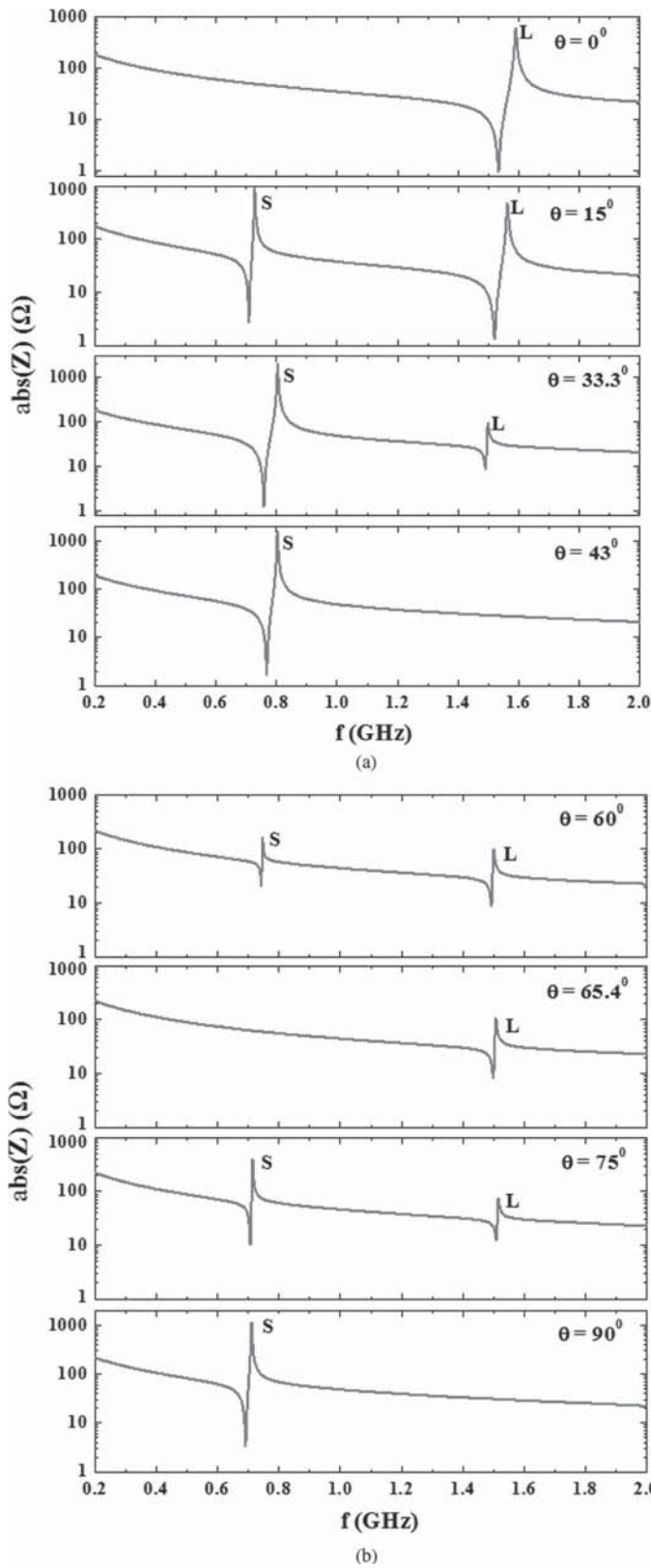
Fig. 6. Impedance spectrum simulation of FBAR based on c-axis tilted ZnO film. (a) \theta = 0, 15, 33.3 , and 43^\circ ; (b) \theta = 60, 65.4, 75 , and 90^\circ .
