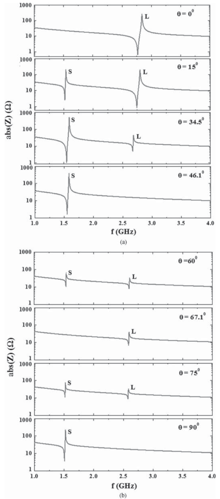
Fig. 7. Impedance spectrum simulation of FBAR based on c-axis tilted AlN film. (a) \theta = 0, 15, 34.5 , and 46.1^\circ ; (b) \theta = 60, 67.1, 75 , and 90^\circ .
