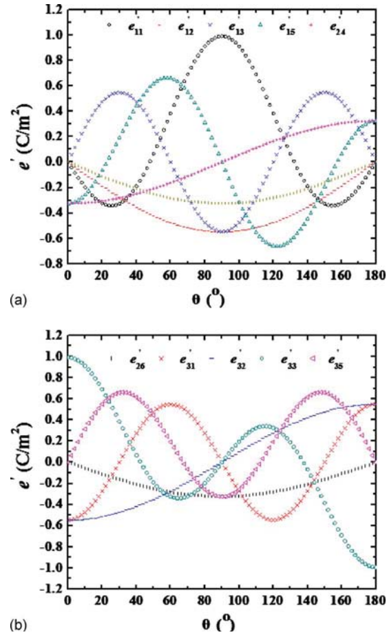
FIG. 5. (Color online) The piezoelectric stress constants ( e' ) of wurtzite GaN thin film as a function of tilt angle.
