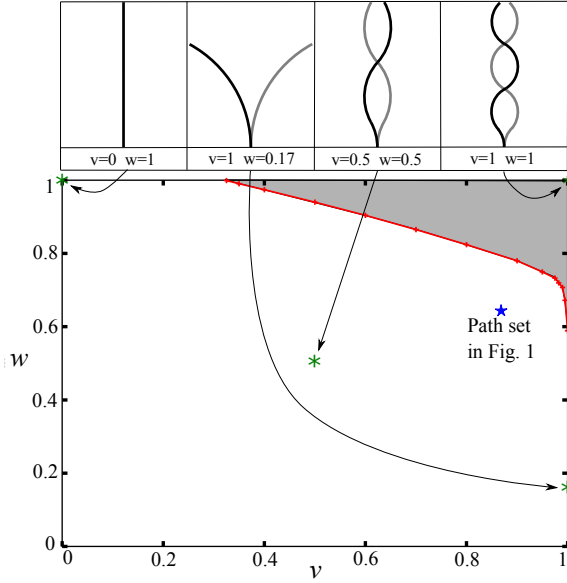
Fig. 4 At top: several example paths combining different values of v and w . Each path pair obeys (3). The value of v affects the “curviness” allowed in paths, while w affects their length. At bottom: this plot, generated numerically, approximates the set of appropriate choices for v and w . The gray region at top right must be avoided, as we show in Lemma 2. Such choices would permit an obstacle to occur between two safe paths that obey (3). A path whose values fall in the white region is called an appropriate path .
