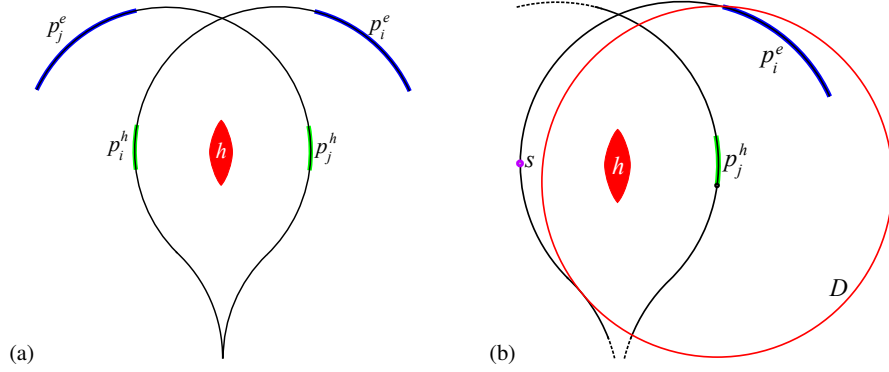
Fig. 8 (a) With bounded curvature, there is a lower bound on path lengths that permit a hole, h , while satisfying (3). Shorter path lengths ensure the existence of a safe continuous deformation between paths. (b) We compute the maximal path length that prevents a hole using Vendittelli's solution to the shortest path for a Dubins car. Starting from the dot marked s , we find the shortest path intersecting the circle D . The interval p_i^e illustrates path lengths permitting a hole to exist.
