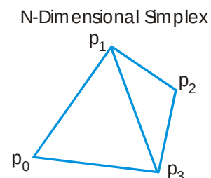
Figure 1: Nelder-Mead uses function evaluation over the vertices of an N -dimensional simplex to optimize a criterion function over an N -dimensional space. Shown here is a tetrahedron, which is a simplex for N=3 . There are N+1 vertices in an N -dimensional simplex.
