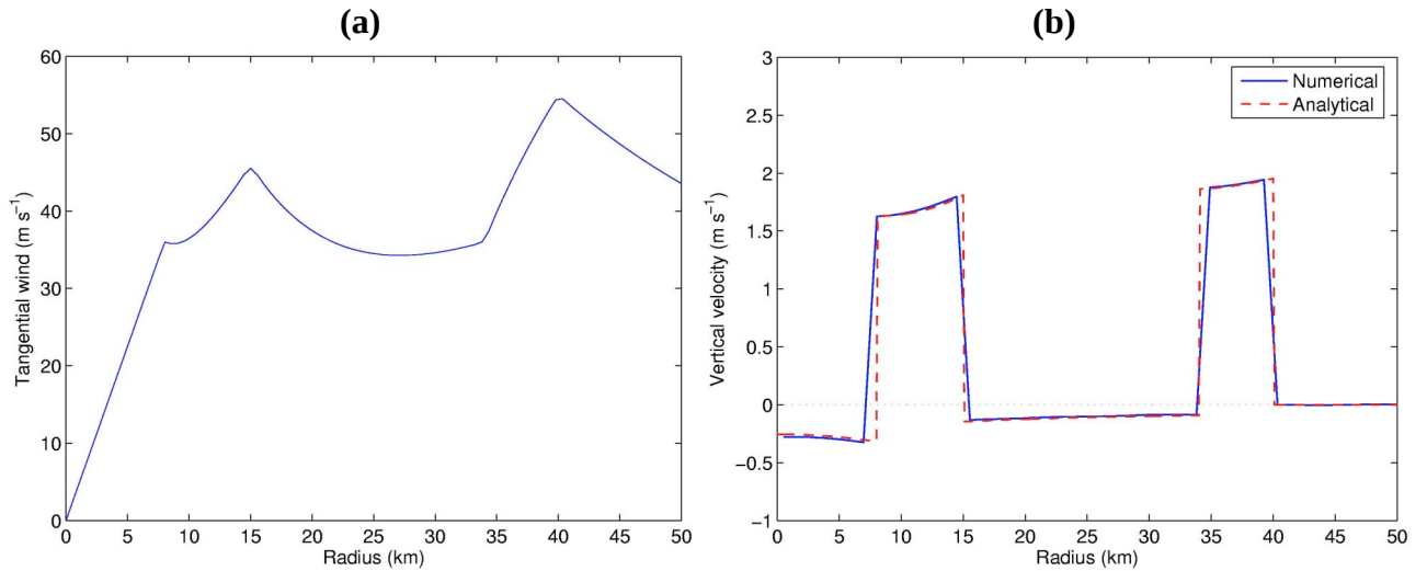
Figure 1. (a) Tangential velocity ( \text{m s}^{-1} ) profile used for the idealized barotropic concentric eyewall and (b) vertical motion ( \text{m s}^{-1} ) from the numerical solution (solid blue) and the analytical solution in Rozoff et al. (2008) at z = 5.9 km.
