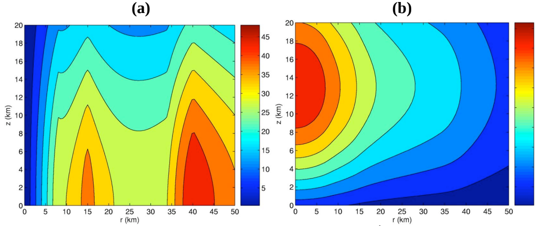
Figure 2. Radial-height cross-sections of (a) tangential wind ( \text{m s}^{-1} ) for the baroclinic vortex and (b) the associated potential temperature anomaly (K) field.
