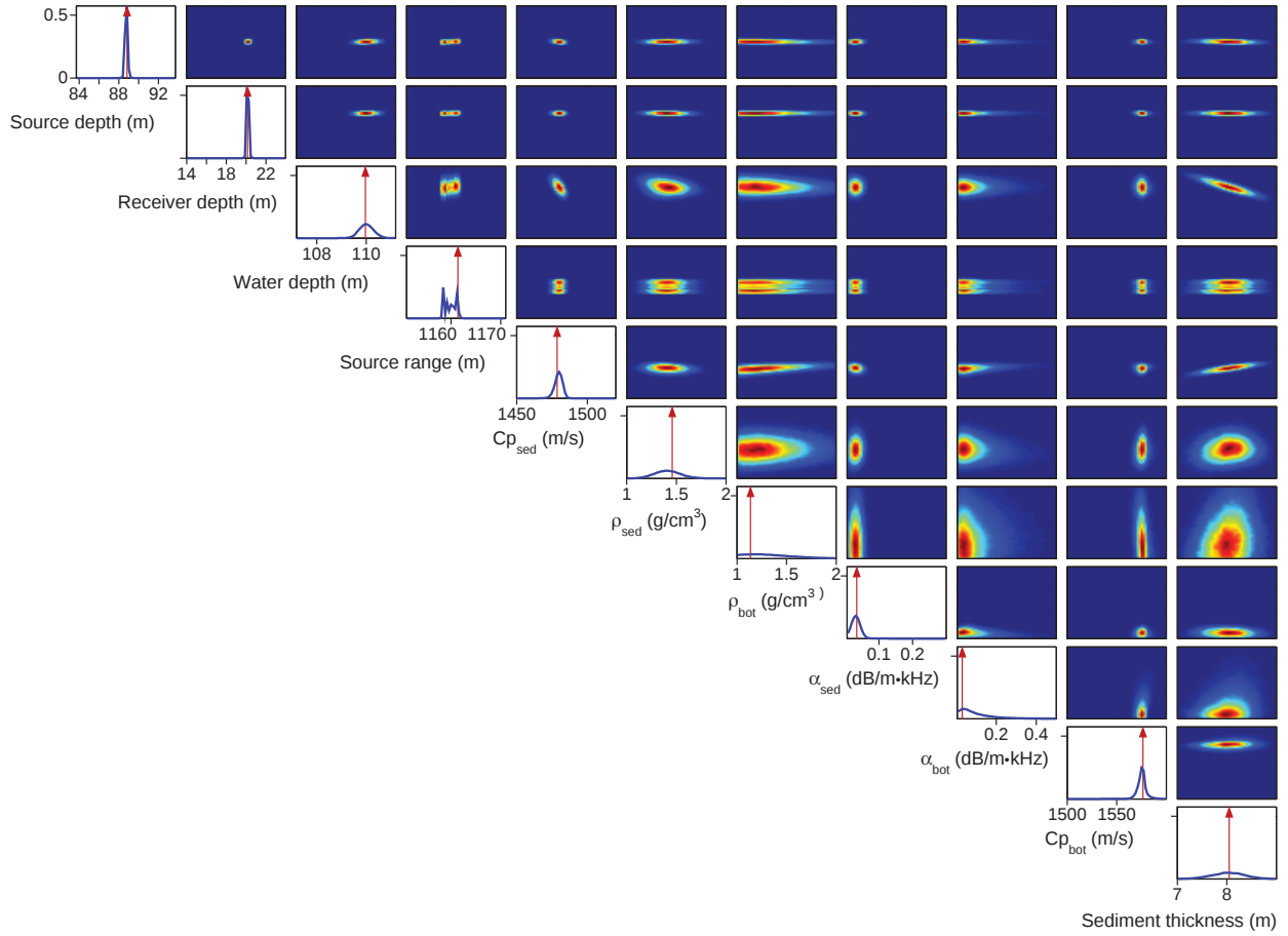
Figure 4. Geoacoustic inversion results obtained from model-based matched filter (MBMF) processing of the sparse array signals shown in Fig. 1(b). The results are presented in the form of 1D-marginal PPD's (line plots) and 2D-joint marginal PPD's (color images) obtained with Bayesian inference for a set of 4 geometrical and 7 geoacoustic parameters.
