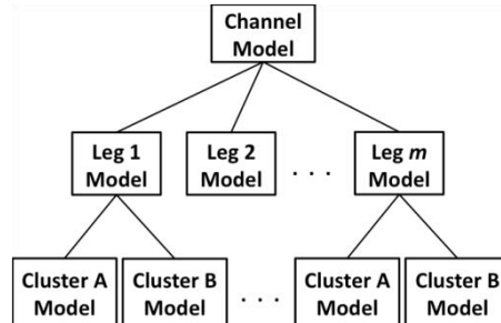
Figure 1. The decomposition of our wireless channel model into component submodels.
