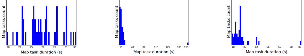
Figure 7. Map task duration distributions. The total number of map tasks is 44 in all three plots. (a) Baseline case, with no exogenous CPU load on node n1. (b) With exogenous CPU load on node n1 but without speculative prefetching. (c) With exogenous CPU load on n1 and with speculative prefetching, the overall map phase completion time is reduced from 213s to 89s.
