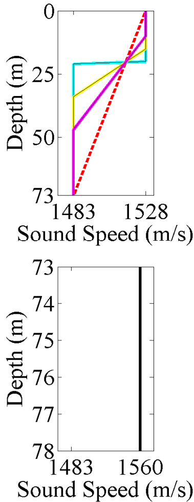
Figure 2. The frequency dependence of modal attenuation coefficients depends mainly on water sound speed profiles in ocean waveguides with sandy-silty sediments and weak range dependence. Upper left panel: Three piecewise-linear thermocline sound speed profiles, each having isospeed segments in the upper and lower water column with values 1528 and 1483 m/sec. The cyan, yellow, and magenta profiles have linear gradients over regions of thickness 1, 19, and 37 m. The dashed red line is a linear profile over the full 73 m water depth. Lower left panel: Sound speed of 1560 m/s in the upper sediment layer, with thickness 5 m and attenuation which is quadratic in frequency. The lower layer is a basement with sound speed 1740 m/s and attenuation which is linear in frequency. Right panel: Log-log plot of modal attenuation coefficients for mode 1, ranging from 0.001 to 1.0 dB/km, versus frequency from 10 to 2000 Hz corresponding to the four water sound speed profiles. The cyan curve decreases steadily and at large frequencies has frequency power-law exponent N of about - 0.9; the yellow curve is similar, with slightly higher attenuation; the magenta curve has decreasing attenuation to about 150 Hz, then increasing slightly to about 400 Hz, and finally decreasing for large frequencies with N = - 0.2 ; the red curve decreases until about 100 Hz and then steadily increases with N = 1.0 . The behavior of modal attenuation coefficients for middle frequencies depends strongly on characteristics of the sound speed profile near the bottom of the water column.
