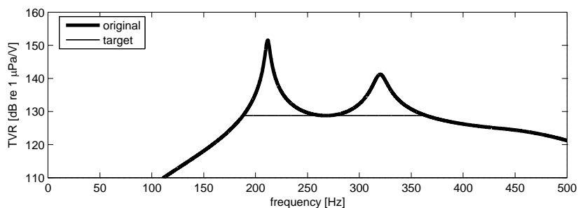
Figure 10. Modeled Multi-Port transmit voltage response (TVR) (heavy black lines). The thin line indicates the reduction goal and pass band after equalization.
