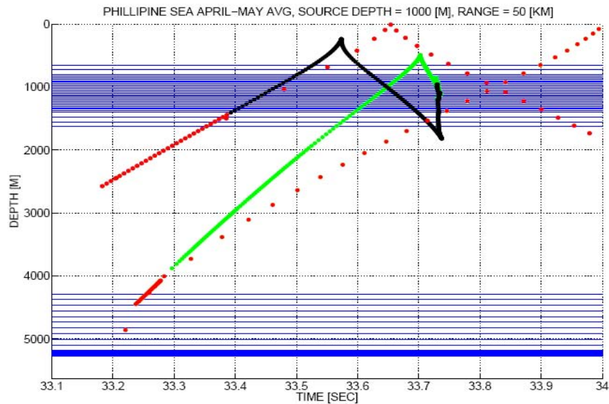
Figure 6. Timefront at 50 km with rays leaving the source at angles between +/- 20 degrees in 0.05 degree increments. Red dots correspond to rays that have reflected off the surface or the bottom, or will reflect before they reach a range of 100 km.
