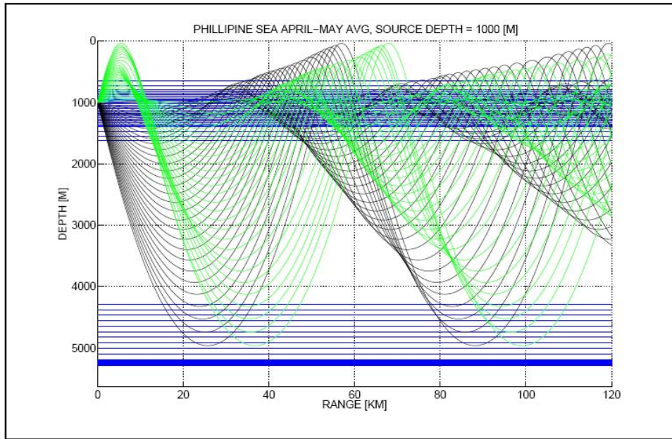
Figure 5. Rays leaving a source at angles of plus and minus 16 degrees from the horizontal. Only rays that do not encounter the surface or bottom are shown. Rays leaving the source with positive angles are shown in green and those with negative angles are shown in black. Blue lines represent planned hydrophone depths. The solid appearing blue band near the bottom is a result of the dense 5-meter spacing here.
