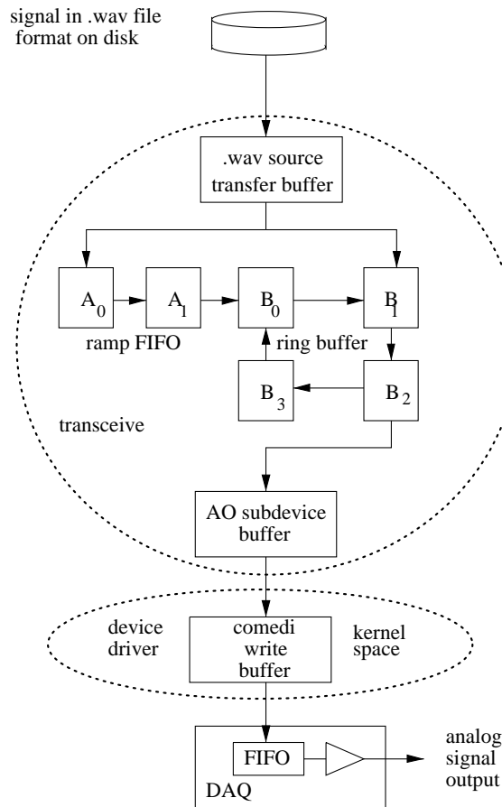
Figure 11. Buffer structure in the transmitter program. The quad ring buffer (B 0 , B 1 , B 2 and B 3 ) supports continuous streaming output for signals of any length. An optional ramp (here, A 0 and A 1 ) can be added to the ring buffer to comply with marine mammal mitigation. The COMEDI write buffer is sized to absorb latencies of more than 1 second while sampling at 10,000 samples per second.
