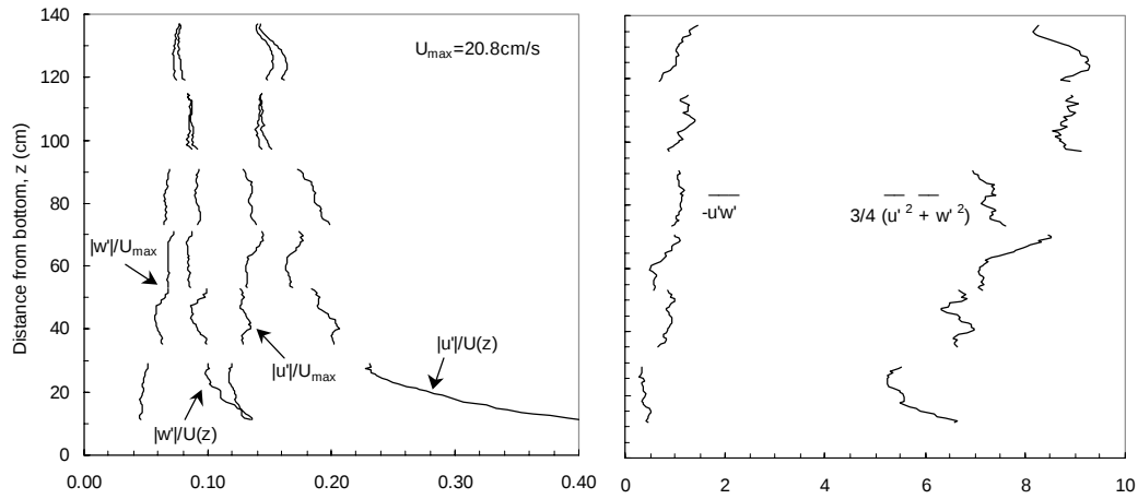
FIGURE 3: (a) Vertical profiles of RMS velocity fluctuations; (b) Vertical profiles of Reynolds stress and estimate for the turbulent kinetic energy, assuming v'=0.5(u'+w') . U_{\max} is the largest value of U(z) ; Averages of u'^2 , w'^2 , u'w' are calculated at constant z , over the entire data set.
