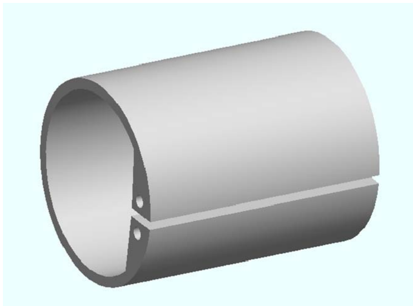
Figure 2. Slotted cylinder geometry used for variable-output projector.
