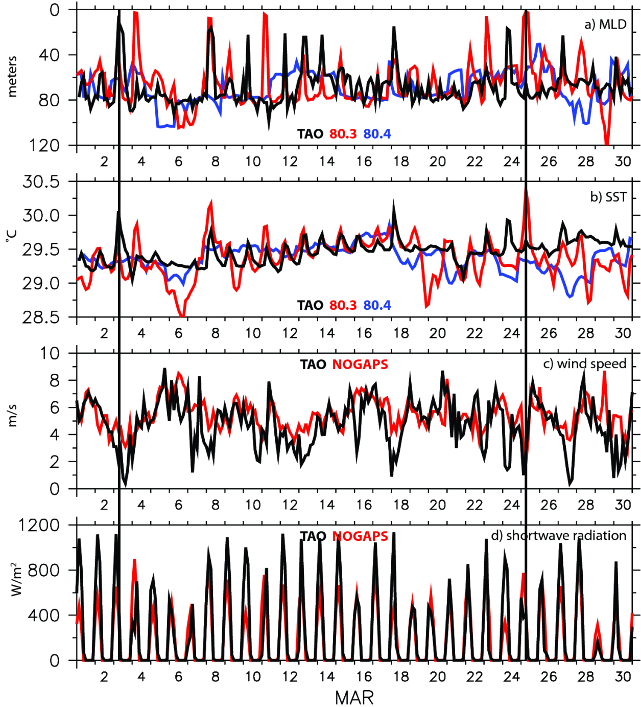
Figure 3: Time series for March 2008 at 137°E, 5°N for a) mixed layer depth (meters), b) sea surface temperature (°C), c) wind speed (m/s) and d) net surface shortwave radiation (W/m 2 ). In panels a, b the black curves are TAO observations, the red curves are hindcast 80.3 with the diurnal cycle and the blue curves are hindcast 80.4 without the diurnal cycle. In panels c, d the black curves are TAO observations and the red curves are from NOGAPS. All curves have 3-hourly temporal frequency.
