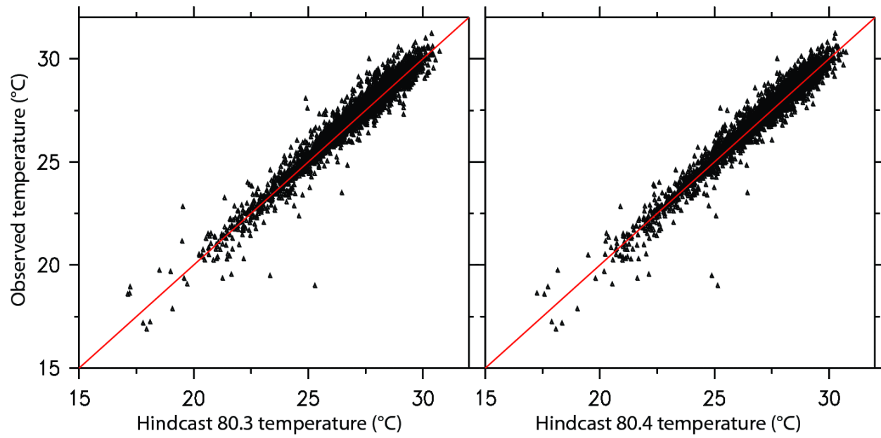
Figure 5: Scatterplot of observed vs. hindcast temperature (°C) at 8 m depth using 4510 unassimilated Argo profiling floats in the MER3c region over the period March-May 2008. Hindcast 80.3 (80.4) is on the left (right) and has a root mean square difference of 0.42°C (0.39°C).
