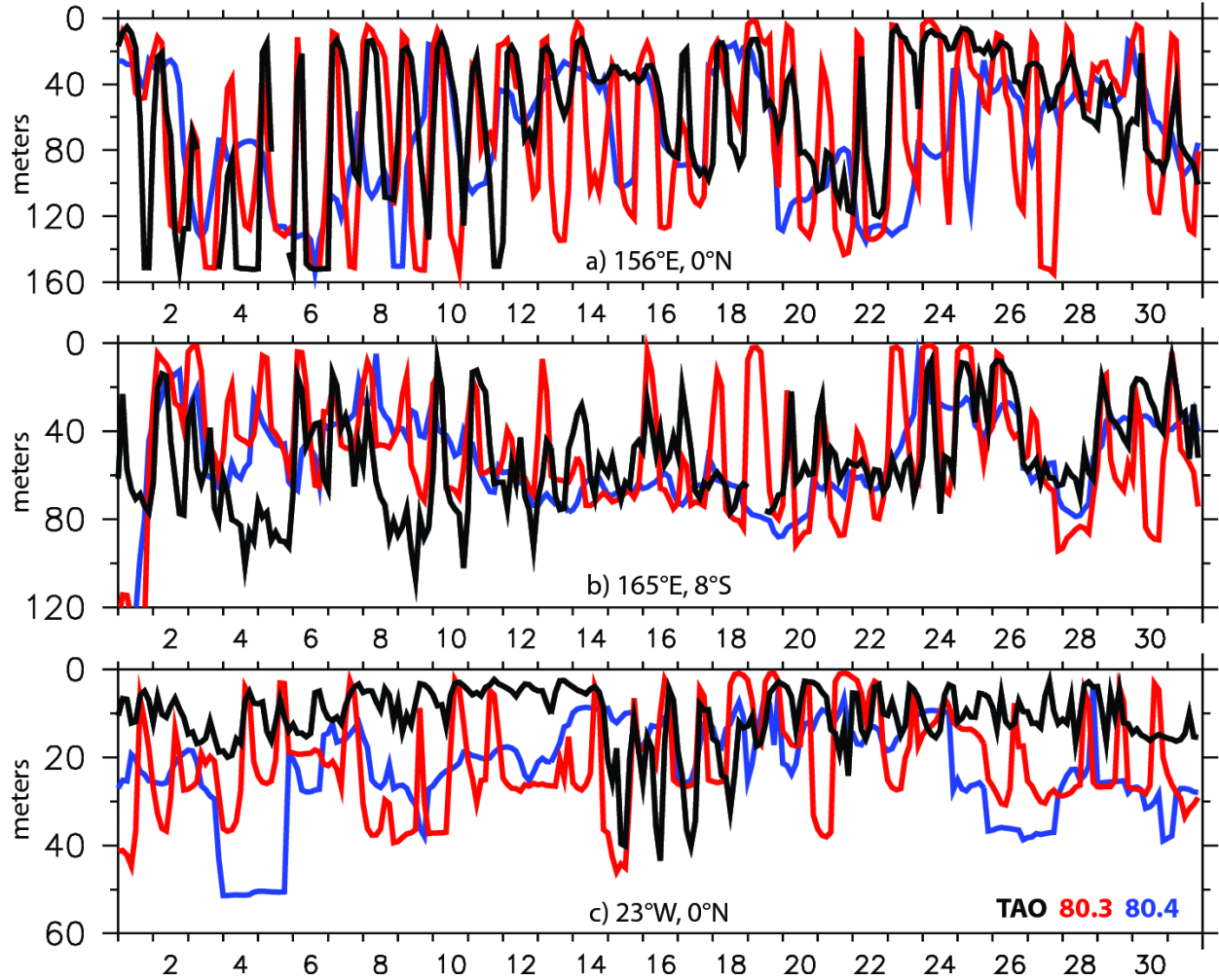
Figure 4: Time series of mixed layer depth (meters) for March 2008 at a) 156°E, 0°N, b) 165°E, 8°S and c) 23°W, 0°N. The black curves are TAO observations, the red curves are hindcast 80.3 with the diurnal cycle and the blue curves are hindcast 80.4 without the diurnal cycle. All curves have 3-hourly temporal frequency.
