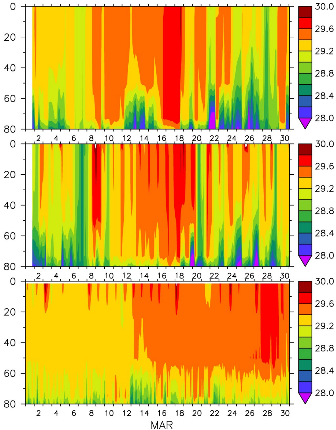
Figure 2: Temperature ( ^{\circ}\text{C} ) vs. depth as a function of time for March 2008 at 137^{\circ}\text{E} , 5^{\circ}\text{N} for hindcast 80.4 without the diurnal cycle (top), hindcast 80.3 with the diurnal cycle (middle) and observations from a TAO buoy (bottom). The tick marks at the bottom mark the beginning of each day and the numbers are marked at the middle of the day. The GOFS V3.0 output are 3-hourly whereas the TAO observations are 1-hourly.
