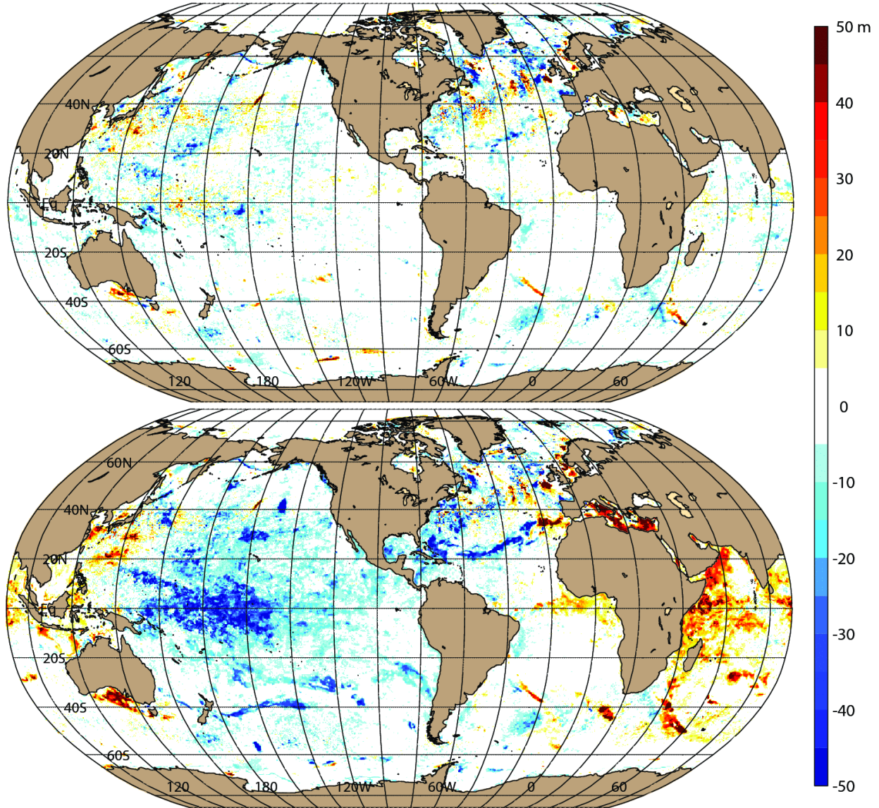
Figure 1: Mixed layer depth difference (in meters) between 15 March 2008 00Z and 15 March 2008 12Z for hindcast 80.4 without the diurnal cycle (top) and hindcast 80.3 with the diurnal cycle (bottom). Values that are less than \pm 5 m are white. The high/low pattern \sim 180^\circ apart rotates around the globe relative to local noon/midnight.
