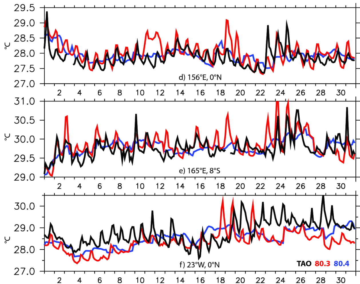
Figure 4 (continued): Time series of SST ( ^{\circ}\text{C} ) for March 2008 at d) 156^{\circ}\text{E} , 0^{\circ}\text{N} , e) 165^{\circ}\text{E} , 8^{\circ}\text{S} and f) 23^{\circ}\text{W} , 0^{\circ}\text{N} . The black curves are TAO observations, the red curves are hindcast 80.3 with the diurnal cycle and the blue curves are hindcast 80.4 without the diurnal cycle. All curves have 3-hourly temporal frequency.
