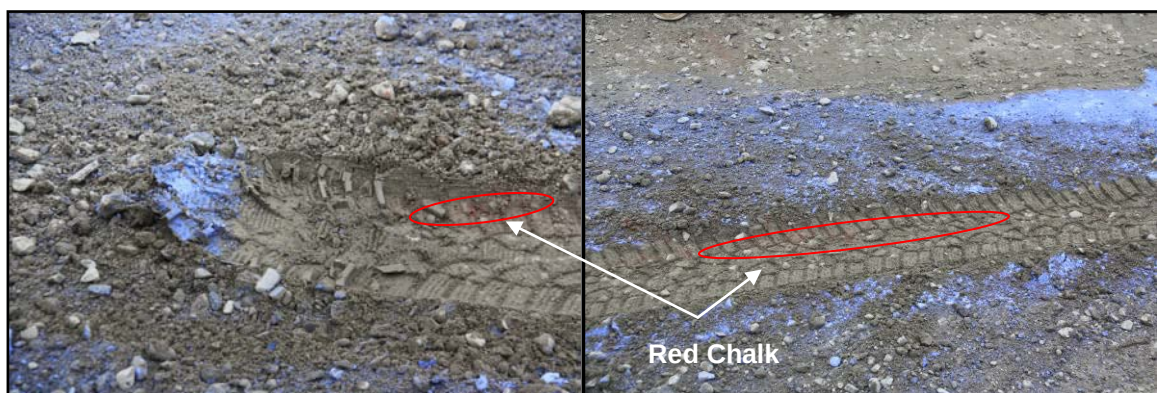
Figure 2. First SLB with Ford Focus at Team O'Neil — Material pushed forward and piled below base of front tire (left) and a small amount of lower red chalk appearing in tire track (right).
