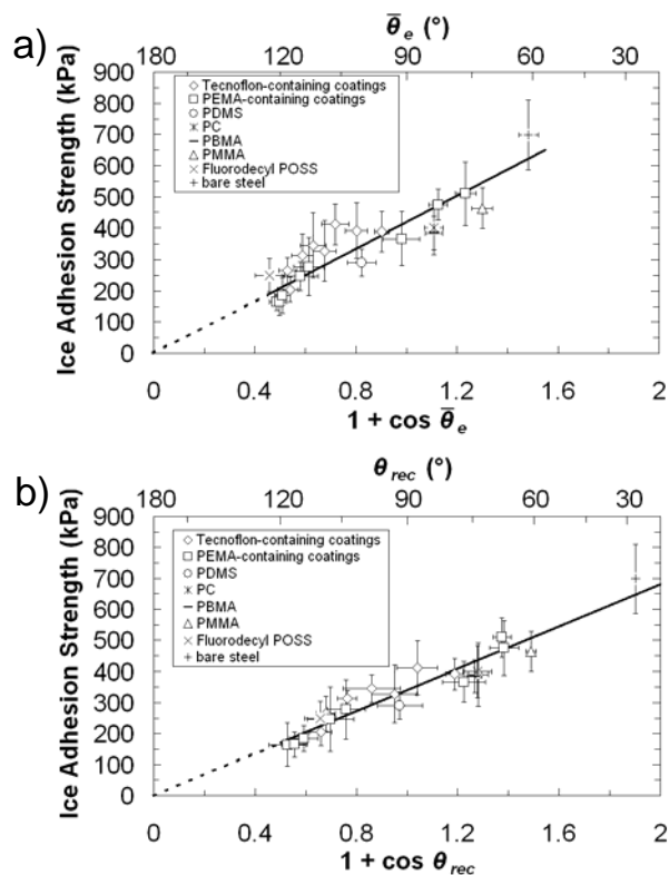
FIGURE 4. Average shear strengths of ice adhesion measured at -10\text{ }^{\circ}\text{C} for bare steel and 21 different coatings plotted against water contact angle parameters that scale with (a) the equilibrium work of adhesion for liquid water (see Equation (2)) and (b) the practical work of adhesion for liquid water (see Equation (3)). The straight lines are the linear best fits that pass through each origin, with the solid portions of the lines encompassing the measured data and the dashed portions representing the extrapolation to the origin. The linear fit for (b) ( \tau_{ice} = (340 \pm 40\text{ kPa})(1 + \cos \theta_{rec}) , R^2 = 0.92 ) is significantly better than that for (a) ( R^2 = 0.80 ).
