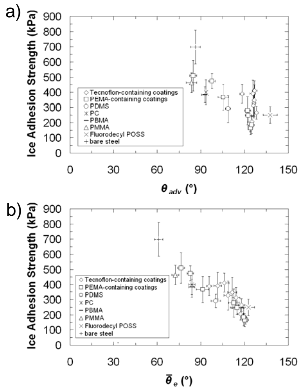
FIGURE 2. Average shear strengths of ice adhesion measured at -10 °C for bare steel and 21 different coatings and plotted against two different measured water contact angles; (a) the advancing water contact angle \theta_{adv} and (b) the estimated equilibrium contact angle \bar{\theta}_e computed using the proposed 60, 81-83 approximation given in Equation (4). Static water contact angles reported in the literature likely fall between \theta_{adv} and \bar{\theta}_e , 81 and these plots facilitate comparison with previous presentations of ice adhesion measurements. 23-25, 31, 34, 42, 43, 51, 53
