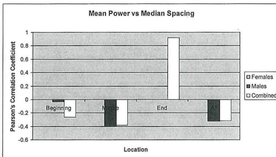
Figure 25. Mean power versus median spacing. Subsets not shown did not occur in data.
