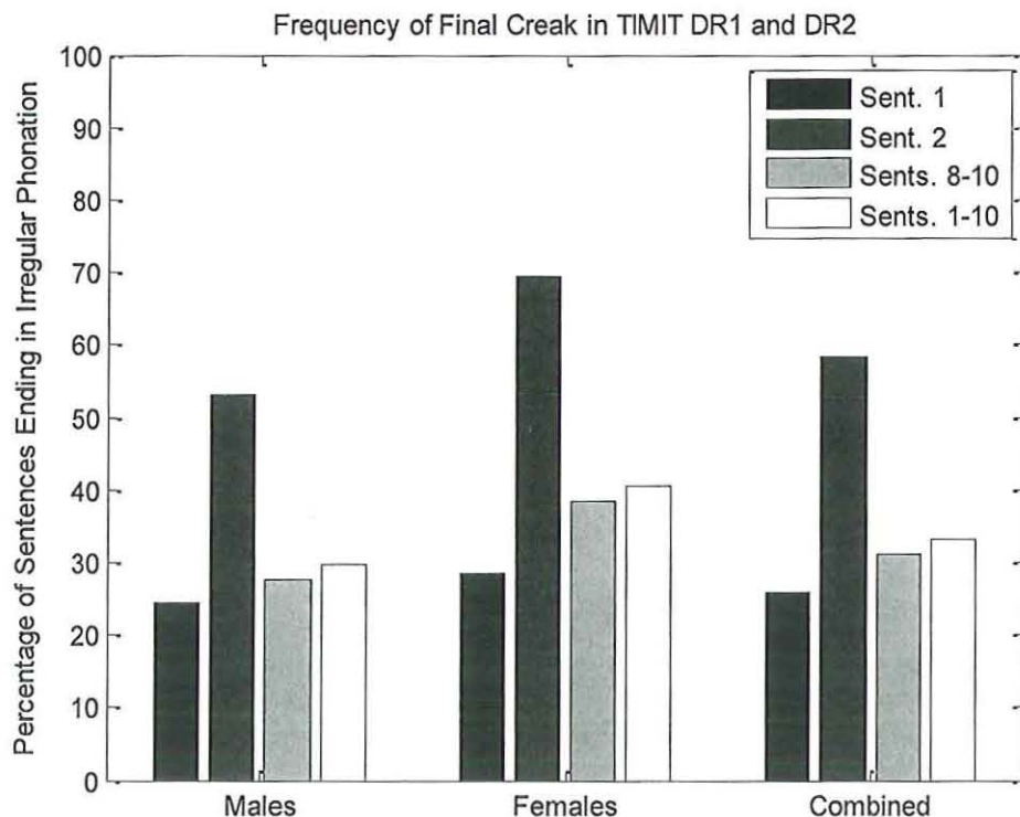
Figure 15. Final creak in the TIMIT population, regions 1 and 2.
