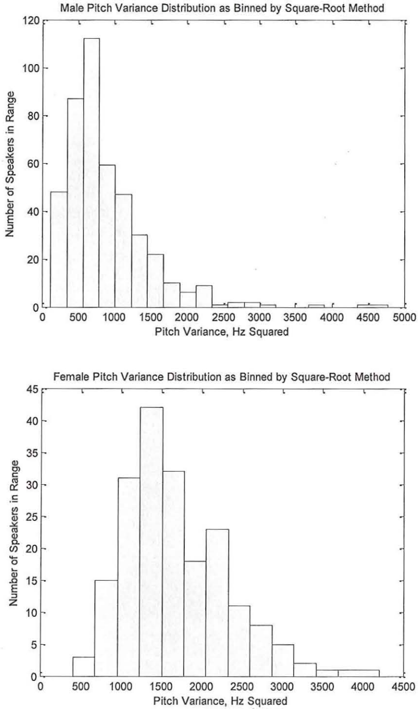
Figure 8. Distribution of variance for males (upper) and females (lower) in TIMIT. For each of the 438 male speakers and 192 female speakers in the database, estimates of the pitch during only voiced regions of speech are obtained as described in Figure 5. For each speaker, we take the variance of the pitch measurements for all samples determined to be voiced in the 10 sentences. This leads to one pitch variance data point per speaker. In this histogram, binning – for which there is no agreed-upon optimal algorithm – is done according to the square-root method, whereby the number of bins in the histogram is equal to the square root of the number of samples.
