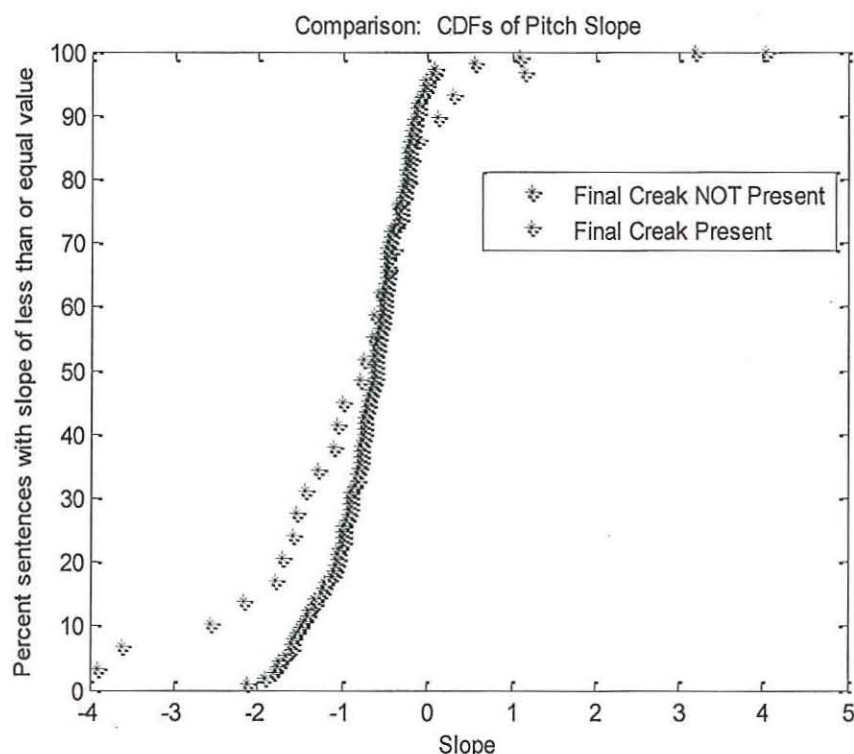
Figure 16. The cumulative distribution function for the approximated slope of the final word of the sentence for cases in which final creak is and is not present. The blue curve indicates the cases in which final creak is not present; the red curve indicates the cases in which final creak is present.
