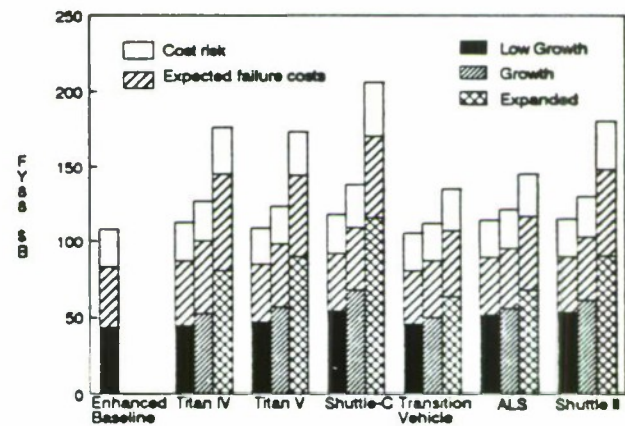
Figure 7-11. – Cost Comparison – All Mission Models
