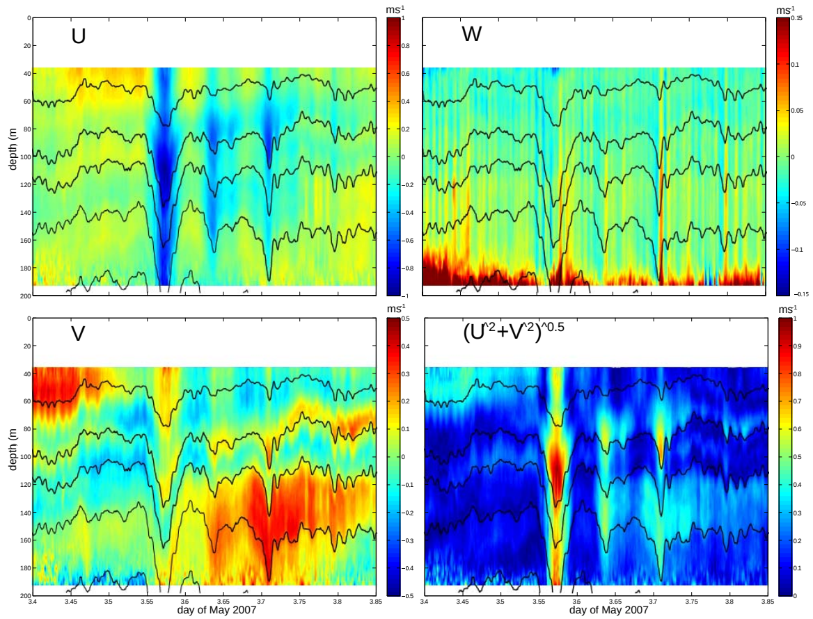
Figure 7. Three-dimensional absolute velocity profiles and horizontal flow speed measured from node 6. The following isotherms are also shown: 25°C, 22.5° C, 20° C, 17.5° C and 15° C. U, V and W are the eastward, northward and vertical upward velocity respectively
