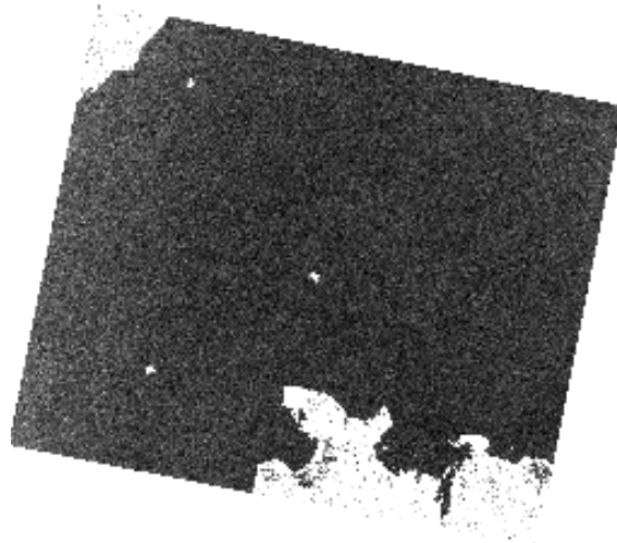
Fig.29. ALOS PALSAR Image over south coast of Negros Island (Date: 2007/10/03, Time: 02:02:59 UTC)
