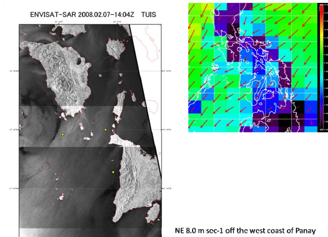
Fig. 7. Sea surface roughness observed by SAR and NCEP wind distribution on Feb. 07, 2008.
