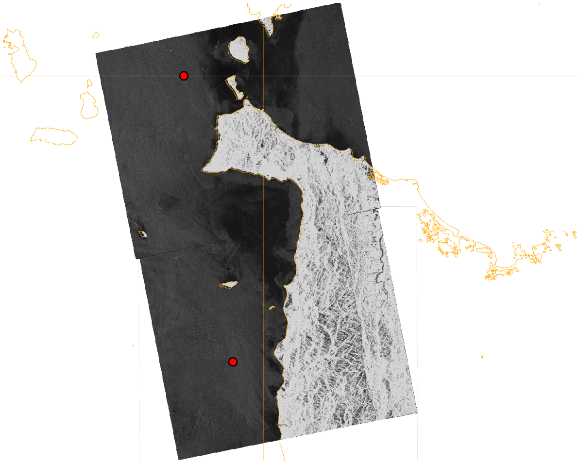
Fig.4 Surface roughness observed by PALSAR on June 21, 2007
