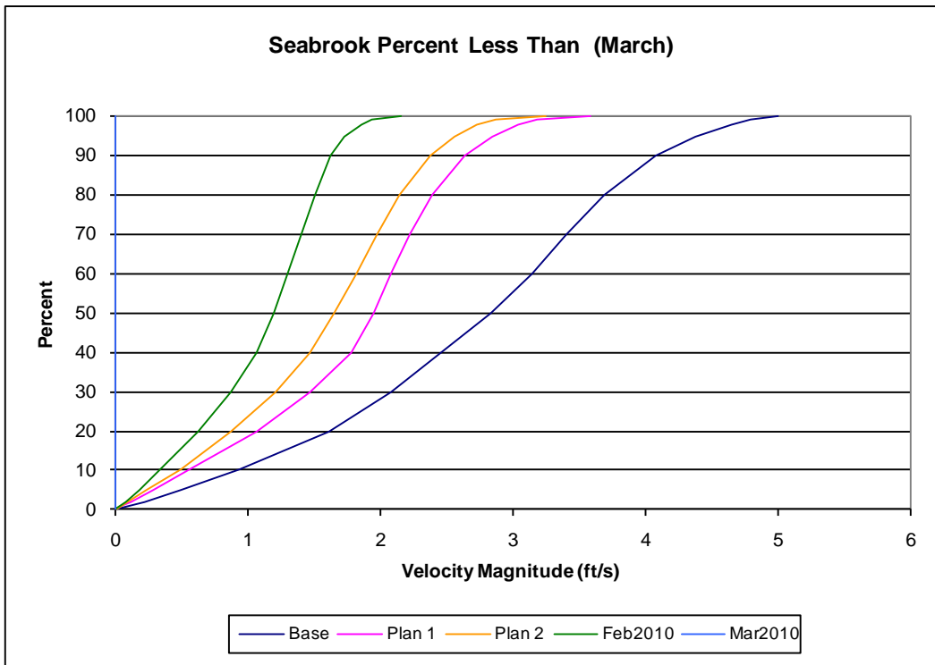
Figure 4-20. Seabrook percent less than plot for March.
