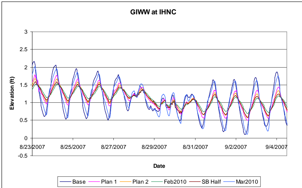
Figure A23. Water surface elevation in GIWW at IHNC (September).
