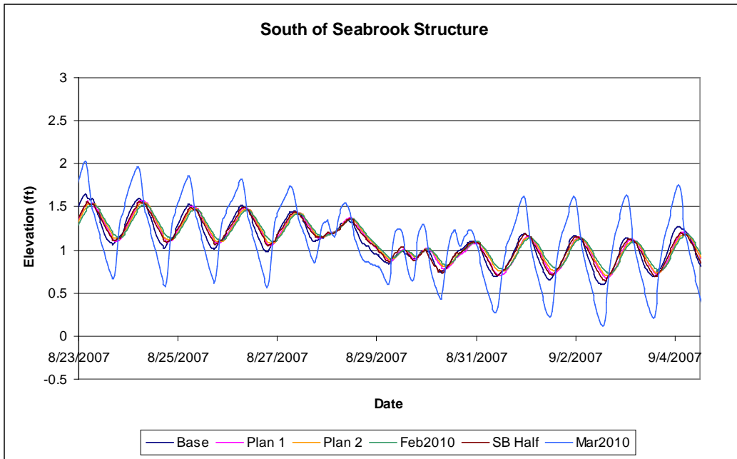
Figure A22. Water surface elevation south of Seabrook structure (September).
