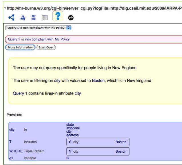
Figure 7. Justification User Interface
