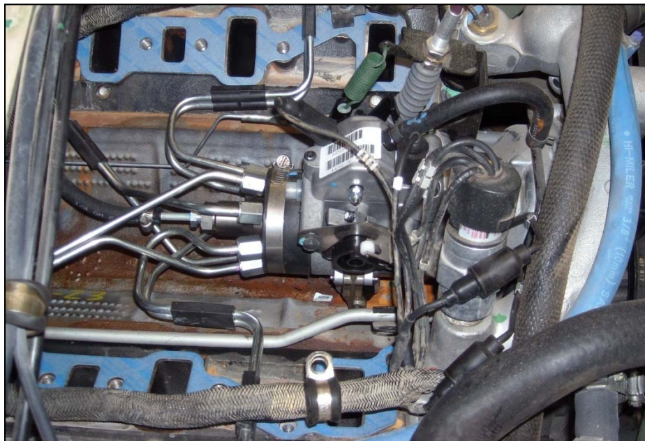
Figure 9 - Newly Installed Stanadyne Rotary Pump
