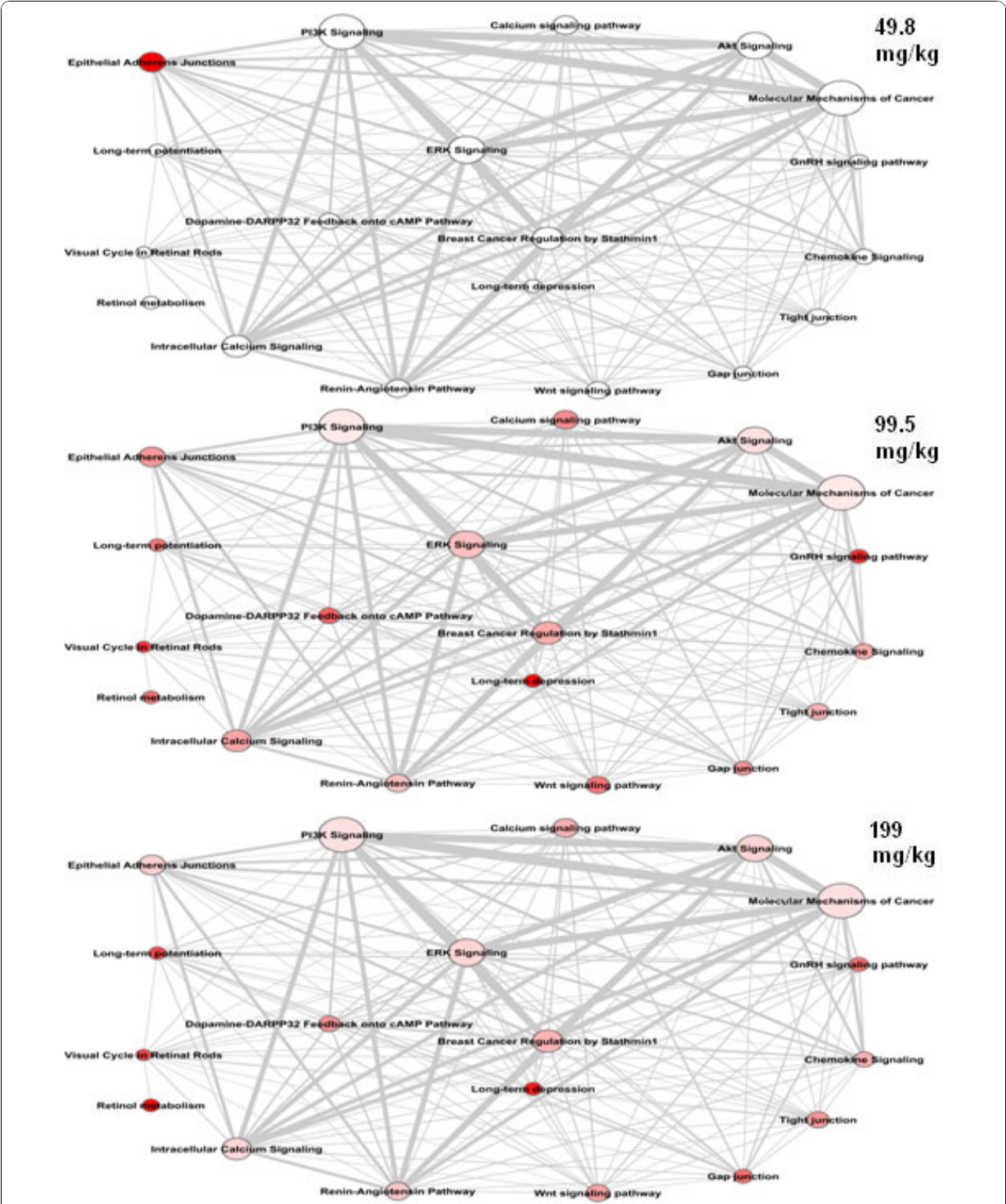
Figure 2 Pathway merging network of top 20 enriched pathways affected by 2,4DNT treatment at each of the three doses. The network was derived from differentially expressed genes (DEGs) across all doses of 2,4DNT. The size of each node is proportional to the number of proteins in a pathway. The color of each node reflects the intensity of the DEGs in each pathway with darker shades of red indicating greater numbers of DEGs. The edge label width is proportional to the number of molecular entities shared by the connected pathways.
