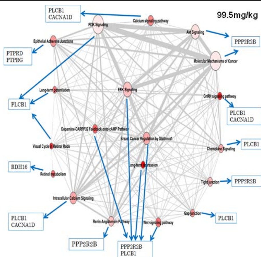
Figure 3 Location of 2,4DNT impacted genes in the pathway association network. Select genes that are differentially expressed in 99.5 mg/kg 2,4DNT exposures are indicated by blue arrows. PPP2R2B = Serine/threonine-protein phosphatase 2A 55 kDa regulatory subunit B beta isoform. PLCB1 = 1-phosphatidylinositol-4,5-bisphosphate phosphodiesterase beta-1. CACNA1D = Voltage-dependent L-type calcium channel subunit alpha-1D. PTPRD = Receptor- type tyrosine-protein phosphatase delta; PTPRG = Receptor-type tyrosine-protein phosphatase gamma. RDH16 = Retinol dehydrogenase 16.
