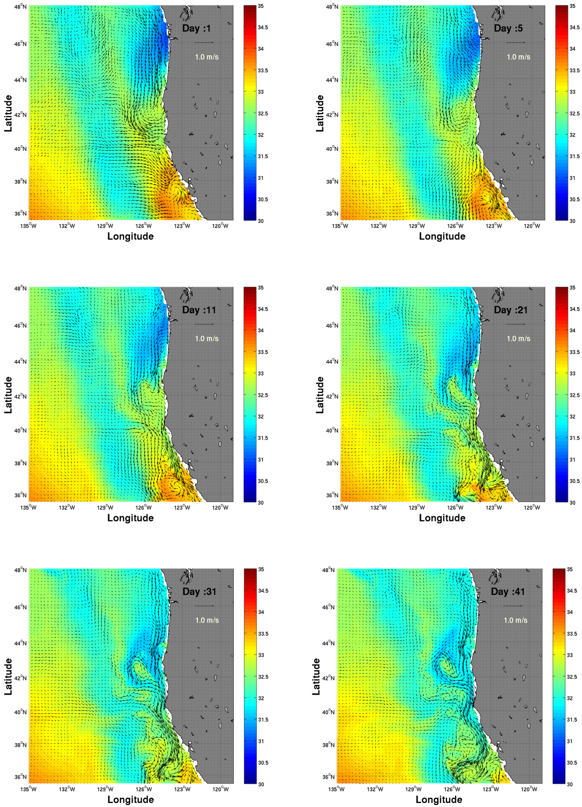
Figure 14. Evolution of 40 days of salinity and velocity fields at surface.
