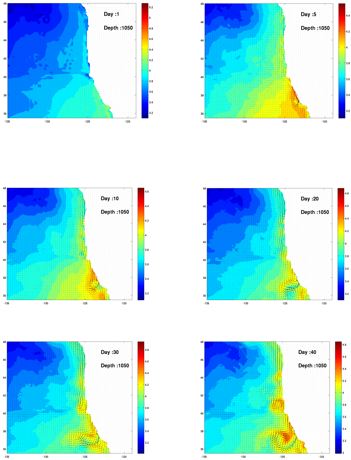
Figure 19. Evolution of 40 days of temperature and velocity fields at 1000m. Sec Section 5.3 for details on the evolution.
