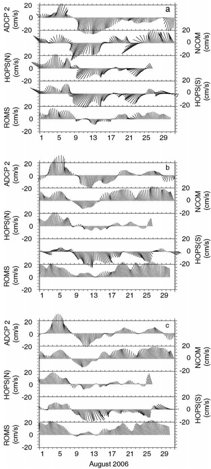
Figure 8. A comparison of currents from ADCP 2 and the four numerical models for: a) near-surface (12 m), b) mid-depth (52 m), and c) near-bottom (72 m).
