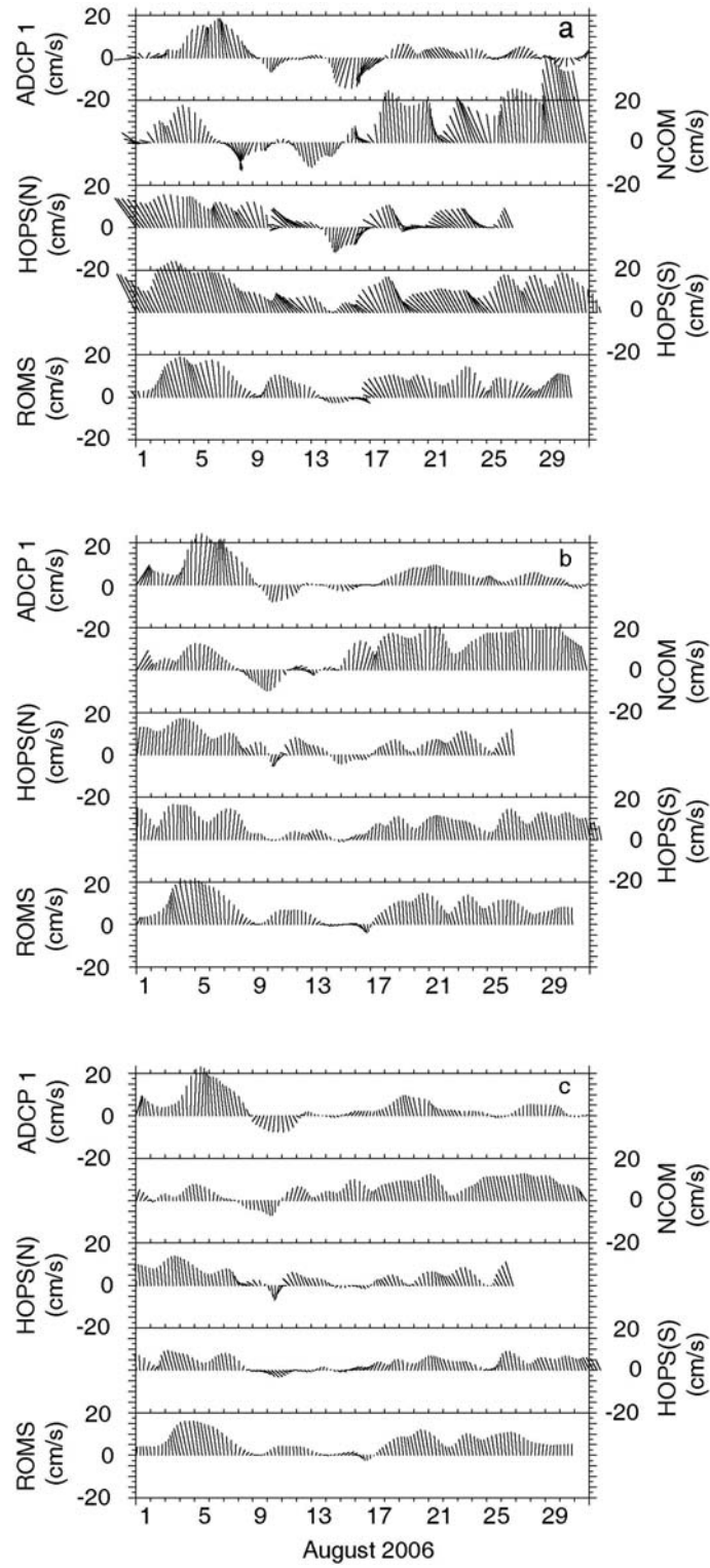
Figure 7. A comparison of currents from ADCP 1 and the four numerical models for: a) near-surface (10 m), b) mid-depth (24 m), and c) near-bottom (46 m). Poleward alongshore is up.
