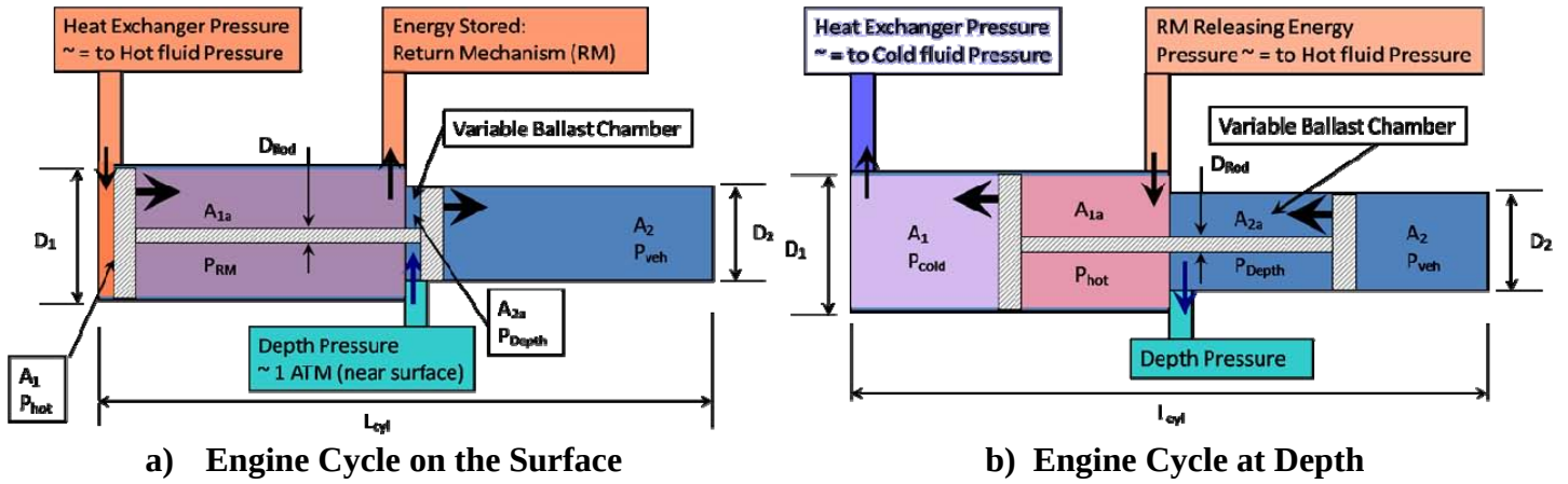
Figure 6. Sketch of Engine Operation at the Surface and at Depth.
