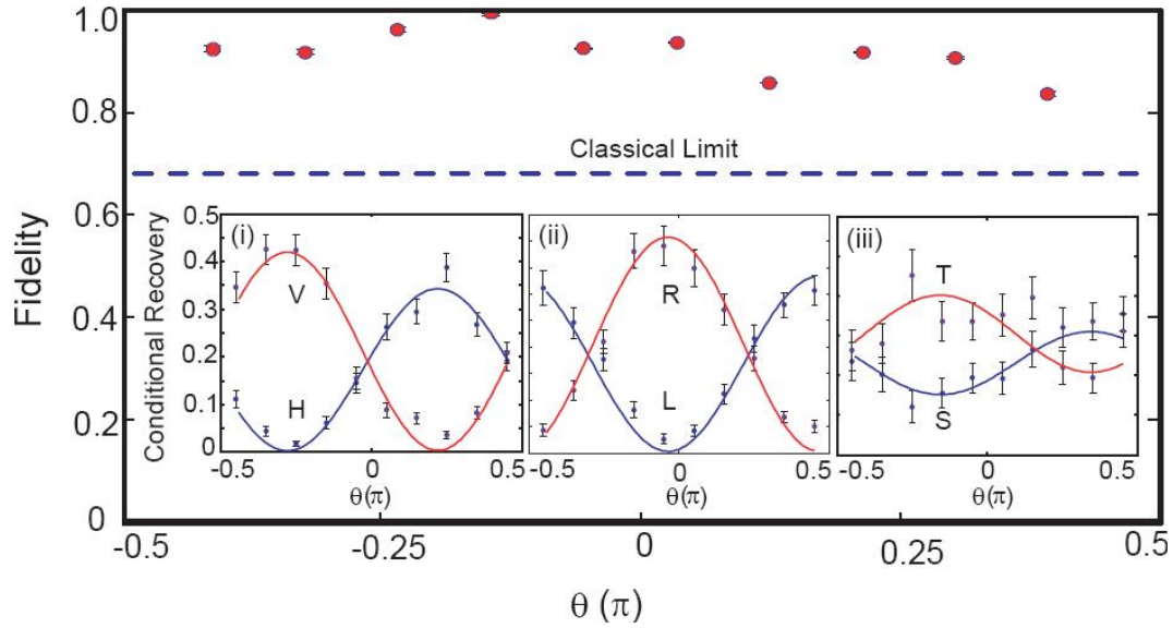
Figure V2. Polarization fidelity of the stored photon as a function of \theta for \phi=0 (Eq. 1). The dashed line indicates the classical limit of 2/3 . Insets (i)-(iii): The results of projection measurements of the output field in three mutually-orthogonal bases, H-V, L-R, and S-T. The solid curves are a simultaneous fit for all sixty data points. The error bars represent statistical errors due to finite detection counts. No backgrounds have been subtracted.
