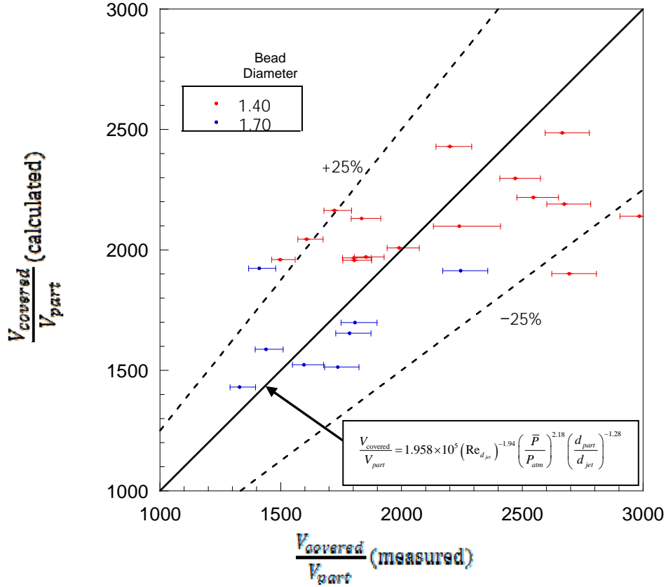
Figure 37: Plot of correlation for calculated versus measured volume of the coated region.
