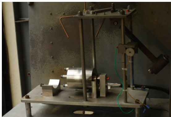
Figure 14: Condensed-phase deposition test rig configuration installed on test stand at HPCL.
