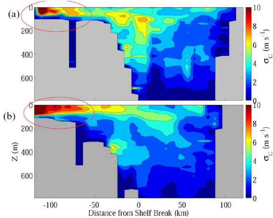
Figure 6: Standard deviations of sound speeds averaged over sections across the continental slope and the continental shelf on possible intrusion paths of the Kuroshio centering around (a) North Mien-Hua Canyon (the top black box in Figure 3) and (b) Mien-Huan Canyon (the bottom black box in Figure 3).
