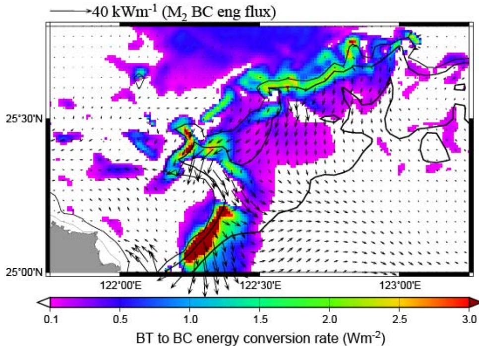
Figure 8: Numerical model results of M2 internal tidal energy flux (vectors) and the M2 barotropic to baroclinic tidal energy conversion rate (color contours). Black contour lines represent isobaths of 200 m, 500 m, and 1000 m.
