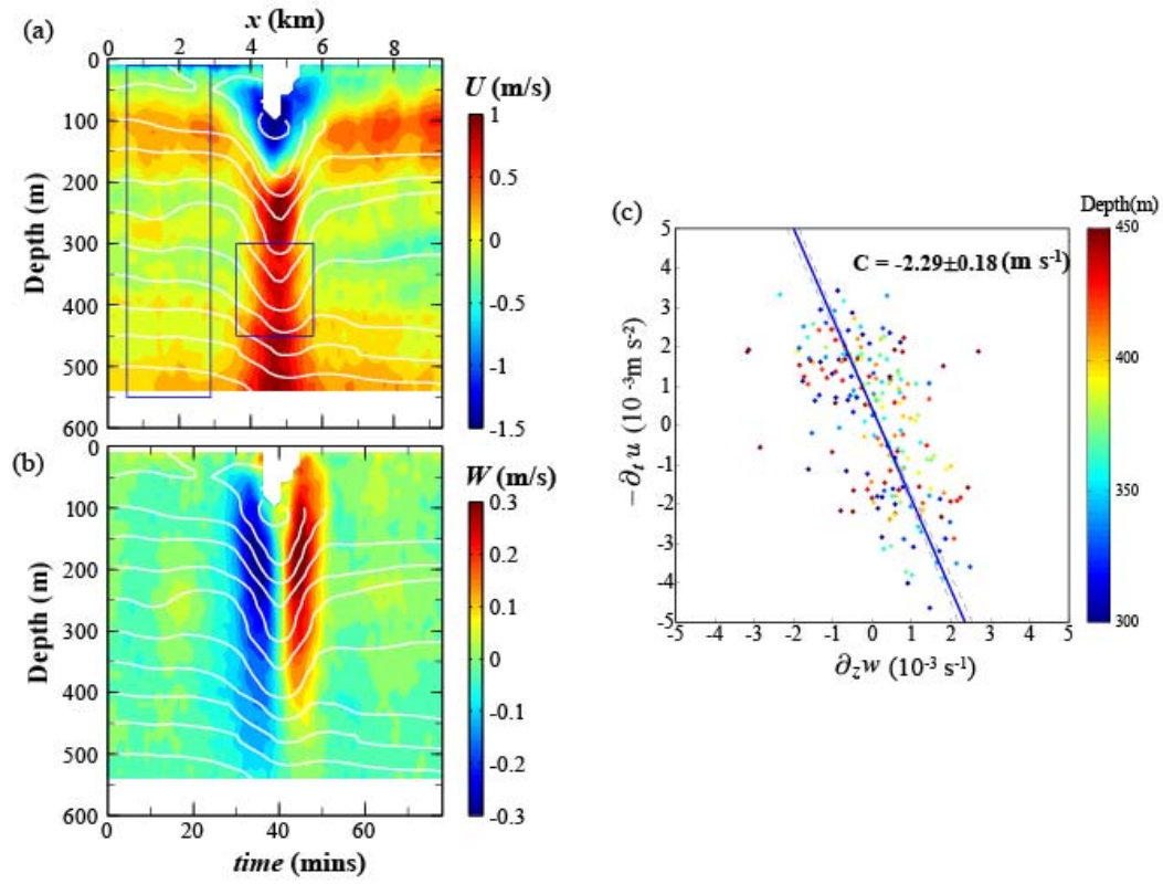
Figure 23: (a) Horizontal velocity and (b) vertical velocity of an observed NLIW event recorded on moored ADCP. (c) Scatter plot of the time rate change of horizontal velocity vs. the vertical divergence of vertical velocity at a 90-s time interval and 16-m vertical resolution. White curves in panels (a) and (b) represent stream lines. The blue lines represent the slope derived by the least square method.
