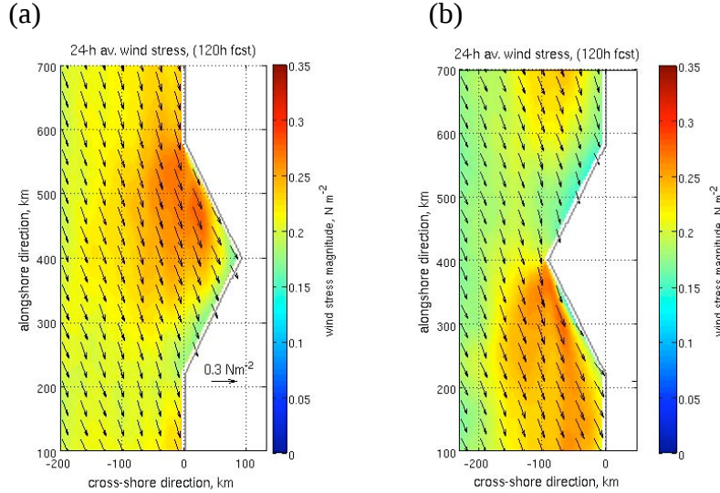
Figure 1. Wind stress (shaded) and wind vectors averaged over 24 hours for a (a) bay, no coupling, and (b) point no coupling. Simulation is 5 days in duration.
