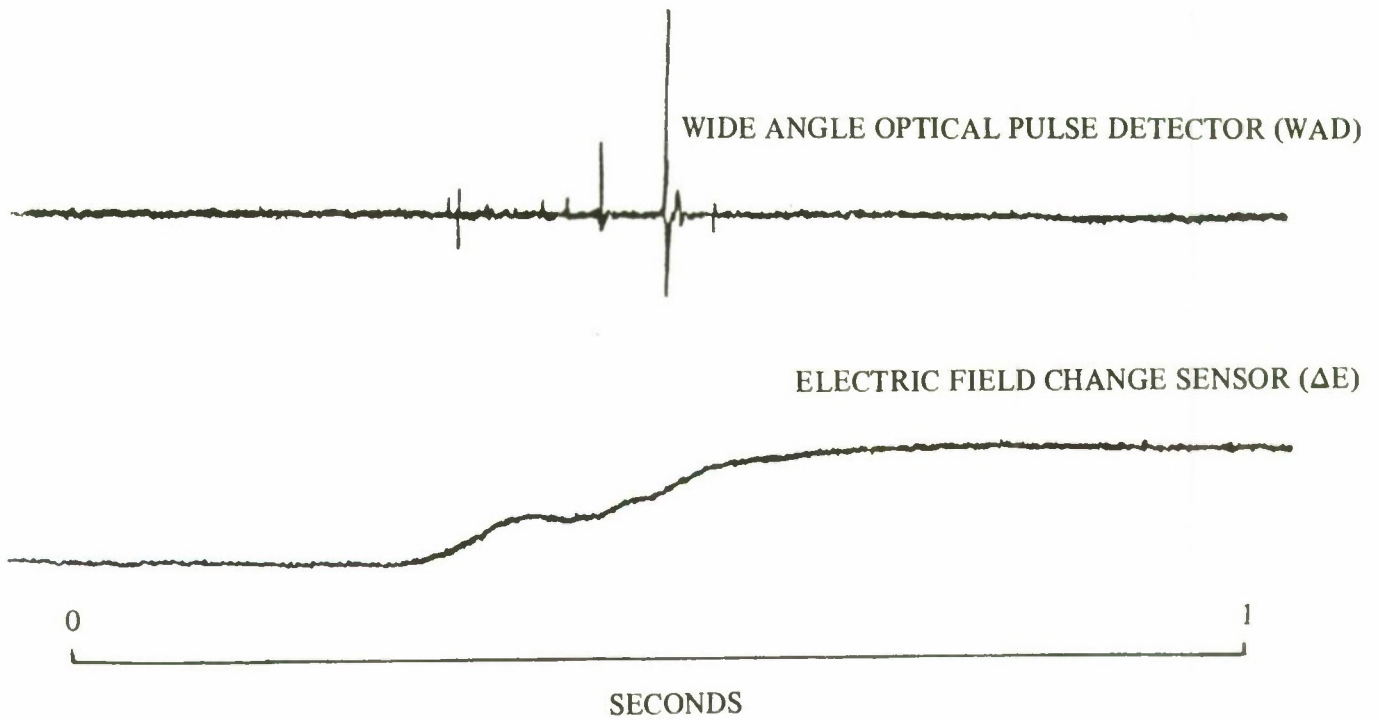
Figure 26. Wide Angle Optical Pulse Detector (WAD) and Electric Field Change Data ( \Delta E ) for August 20, 1983 GMT 031111.
