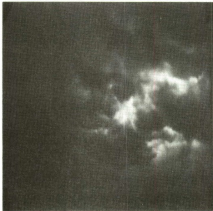
Figure B-4. August 19, 1982, GMT 033058, Flight No. 4, Cloud Top/Lightning Flash.
