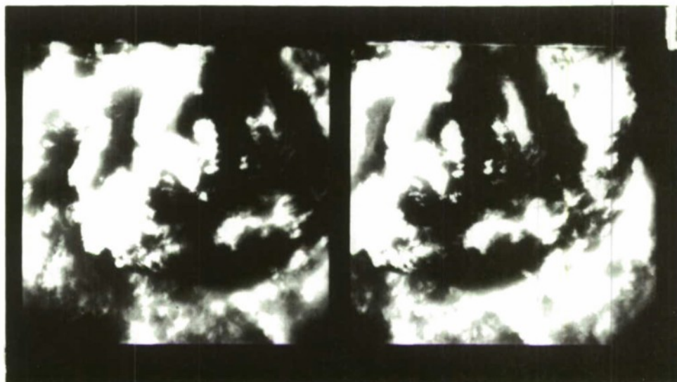
Figure A-9. May 22, 1982 GMT 001648-001634. 48 optical pulses sensed by OPD (time period 4.38 sec, 3 events) during this flight time.
