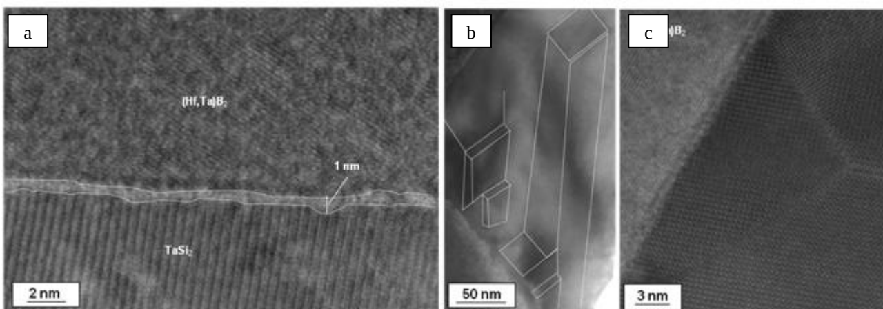
Fig. 9: (a) High-resolution TEM image showing an example of wetted grain boundary at the (\text{Hf,Ta})\text{B}_2/\text{TaSi}_2 interface. (b,c) Twins crystallization in the \text{Ta}_5\text{Si}_3\text{B}_2 phase which displays non-wetting behavior towards the solid solution under this orientation.
