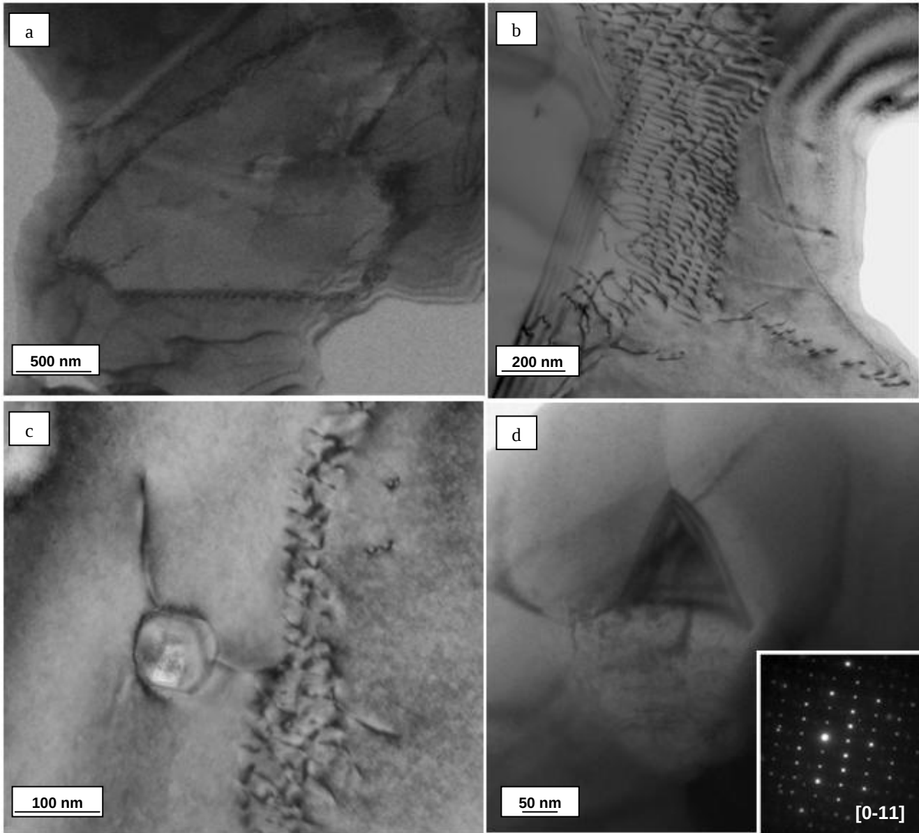
Fig. 3: Bright field TEM images showing a) a typical \text{ZrB}_2 grain surrounded by (\text{Zr,Ta})\text{B}_2 solid solution, b) dislocations in the solid solution, c) a crystalline SiC particles within amorphous Si-O phase from which a dislocation departs and d) the \text{Ta}_{4.8}\text{Si}_3\text{C}_{0.3} phase at the triple point.
