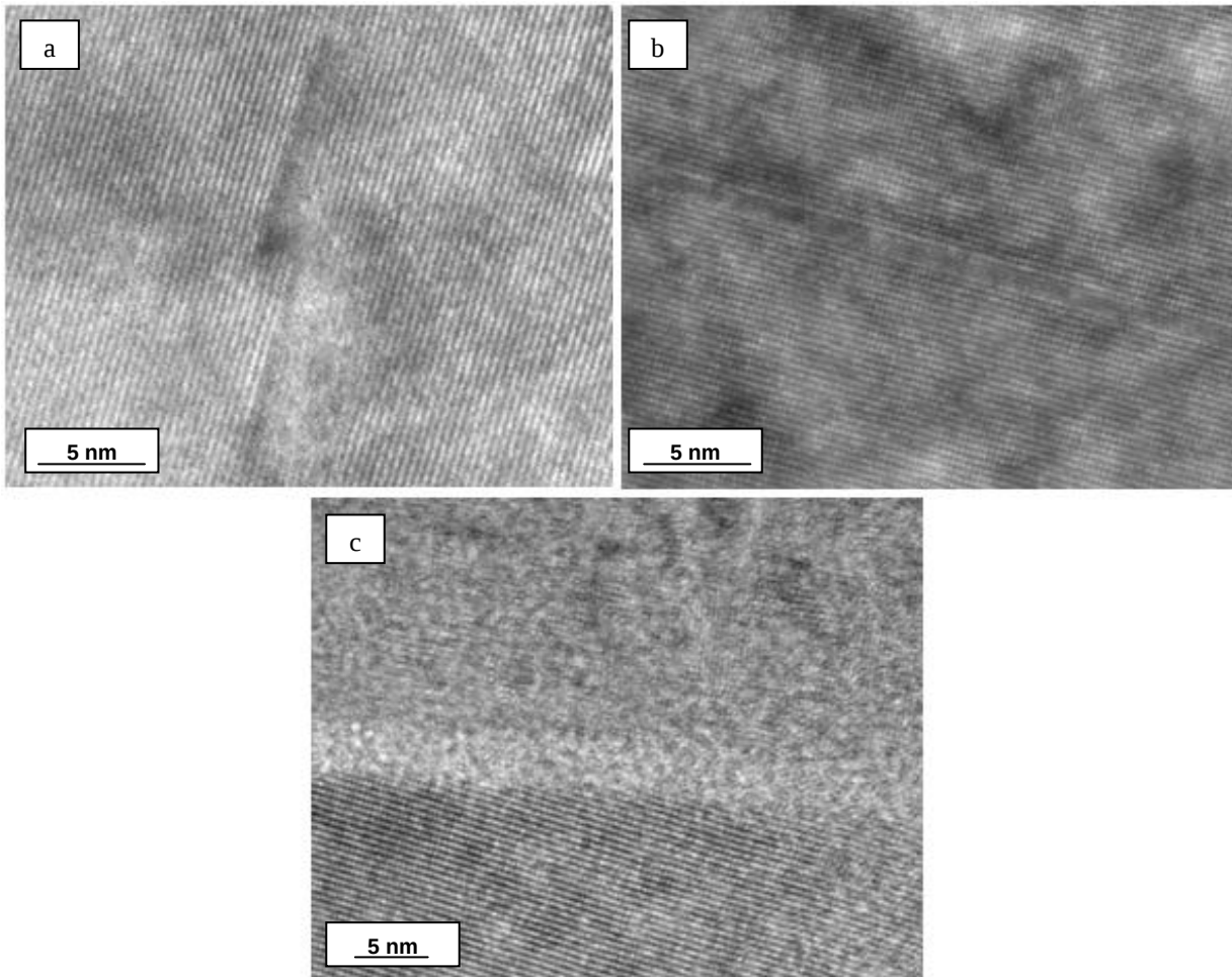
Fig. 5: (a) Stacking faults in the solid solution, (b) interface between core and shell showing low angle grain boundary, (c) example of wetted grain boundary between two adjacent (\text{Zr,Ta})\text{B}_2 grains.
